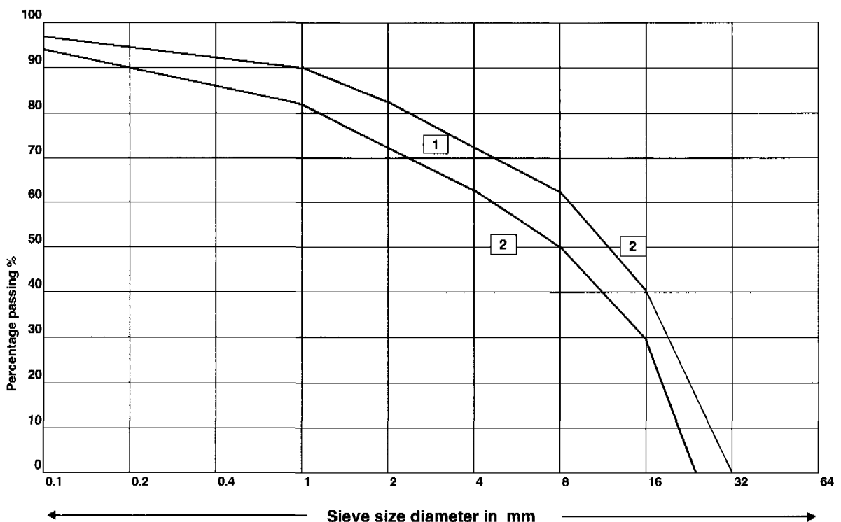
Grading curve 0 - 32 mm
