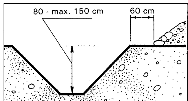
loose ground correct excavation
