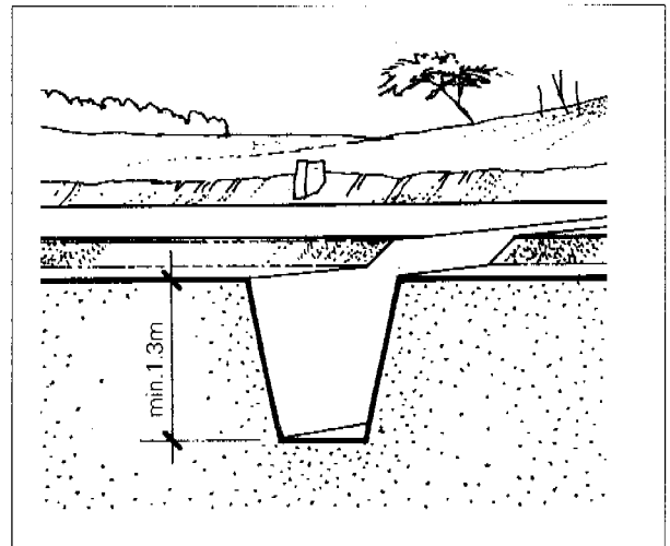
road crossings min. 1.3 m
