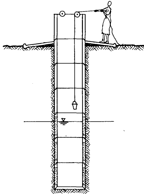
Windlass:
