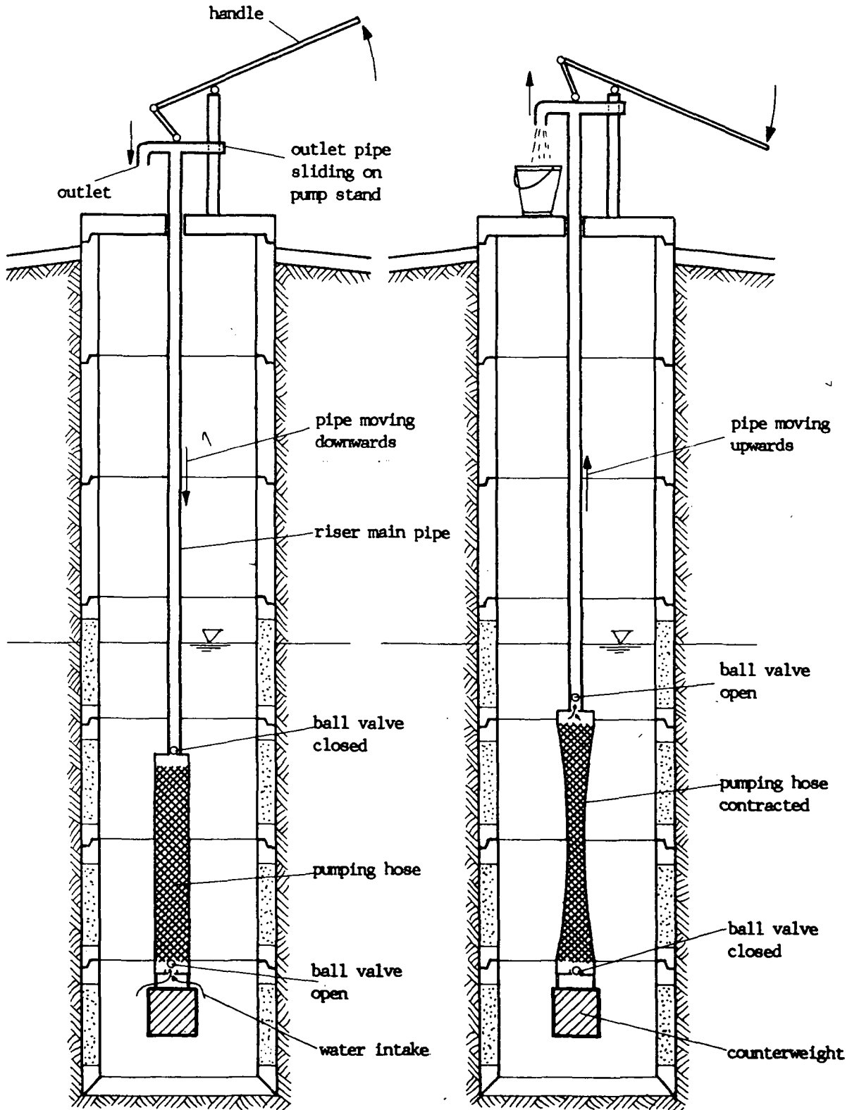
Schematic Illustration
