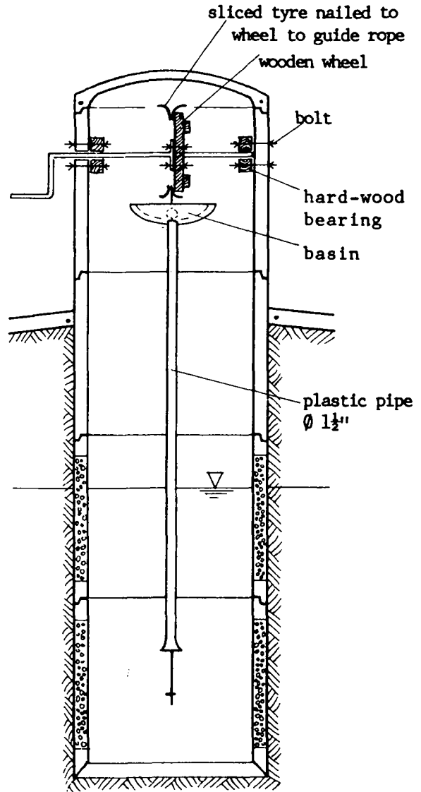
CROSS-SECTION B-B
