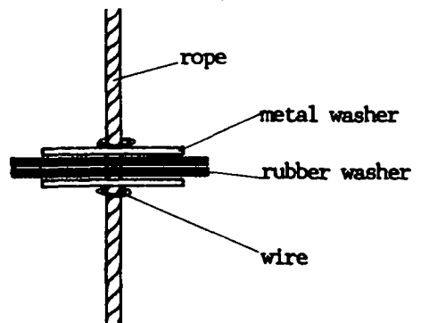
DETAIL: ROPE AND WASHER
