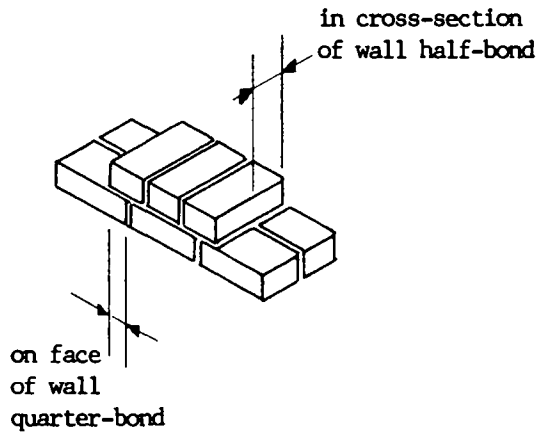
One-Brick Wall
