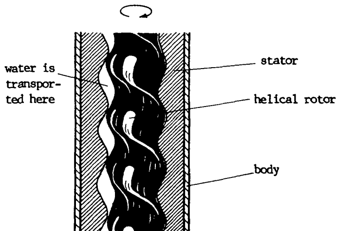
DETAIL OF PUMPING ELEMENT
