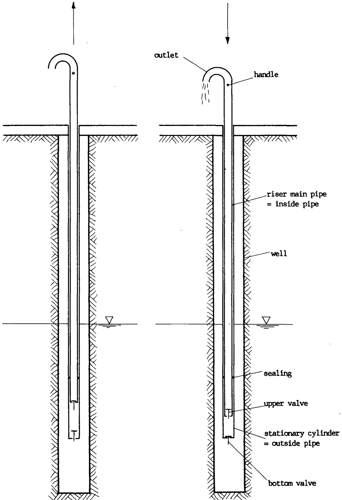
Schematic Illustration
