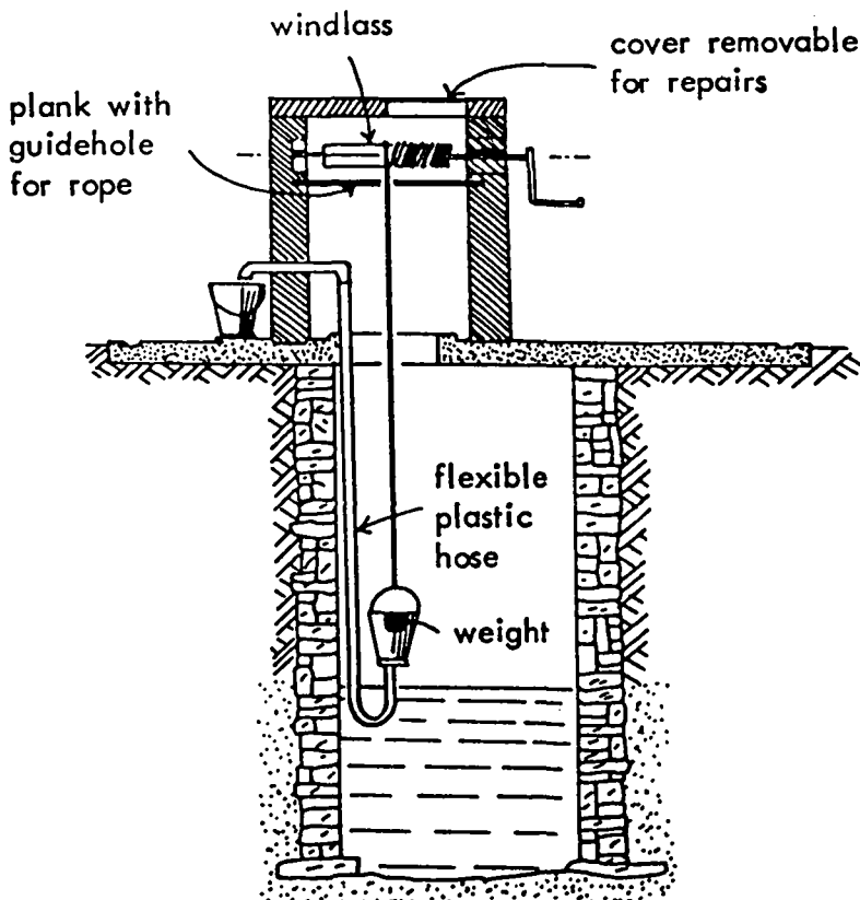
Schematic Illustration
