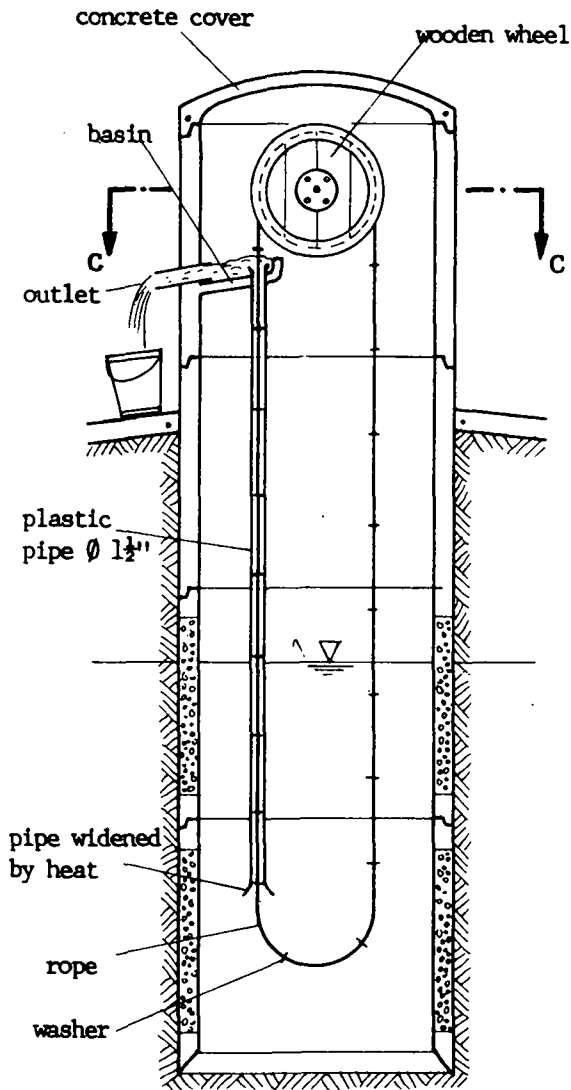
CROSS-SECTION A-A
