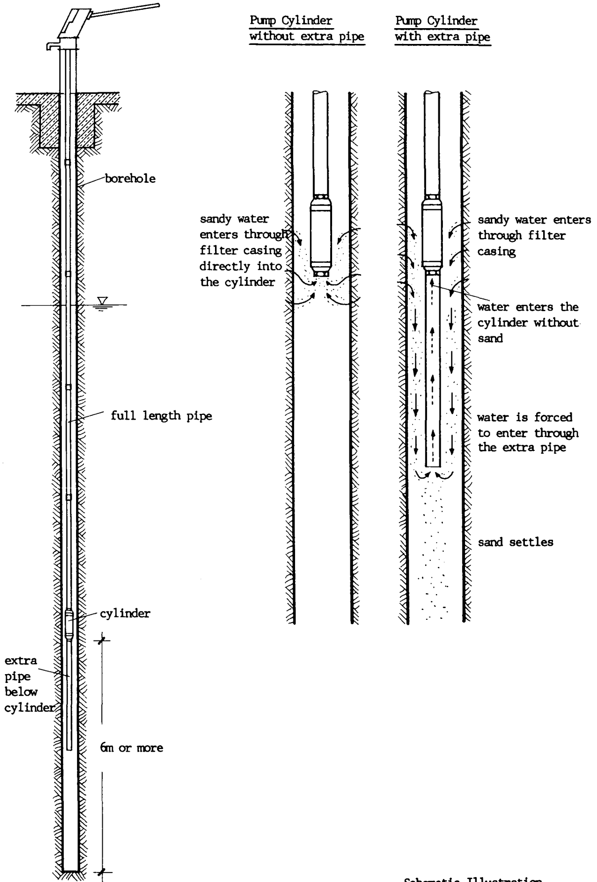
Schematic Illustration
