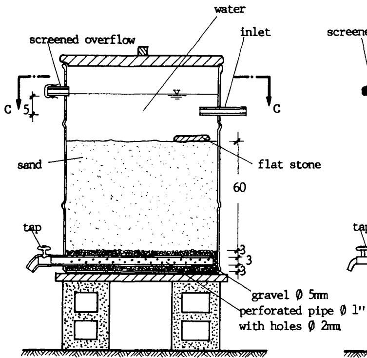
CROSS-SECTION A-A
