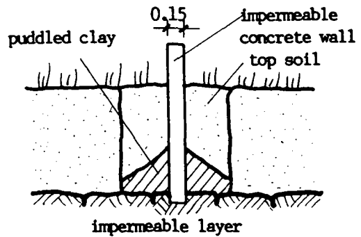
CROSS-SECTION B-B: ANTI-SEEPAGE WALL
