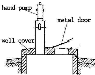
Manhole with metal door:
