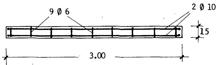
LAYOUT PLAN C-C (1:40)
