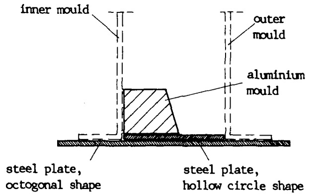
Cross-section A-A through base plate
