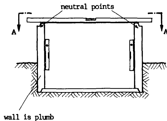
CROSS-SECTION C-C
