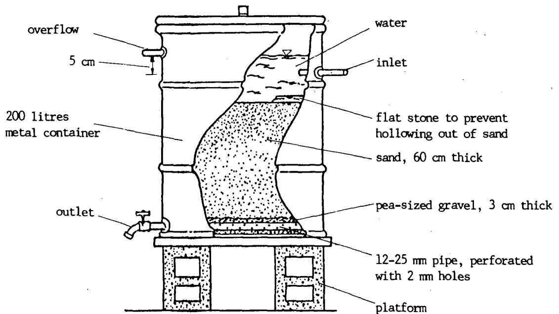
Example: Household Sand Filter
