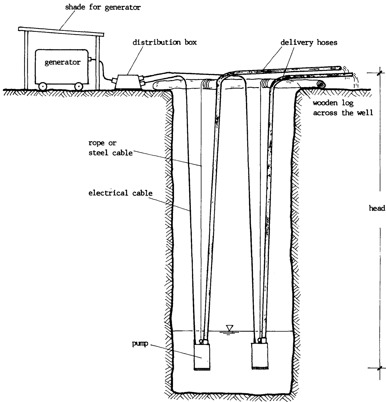
Schematic Illustration
