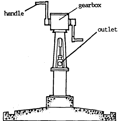
CUT-AWAY SIDE-VIEW
