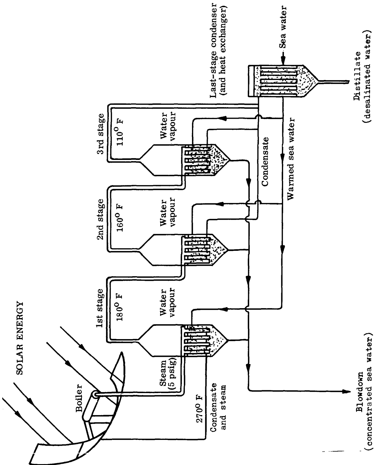
Figure 19. Multiple-effect evaporator heated by steam from focusing solar collector
