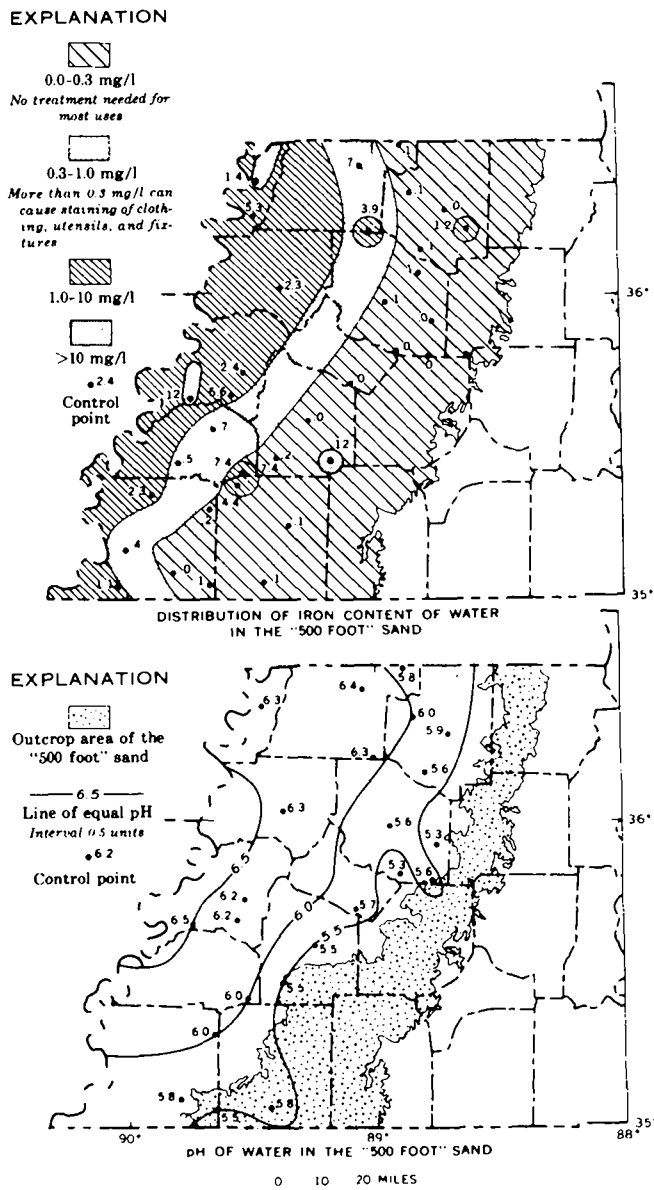
Figure 42. Distribution of iron and pH in water from the "500 foot" sand, western Tennessee (Moore, 1965).
