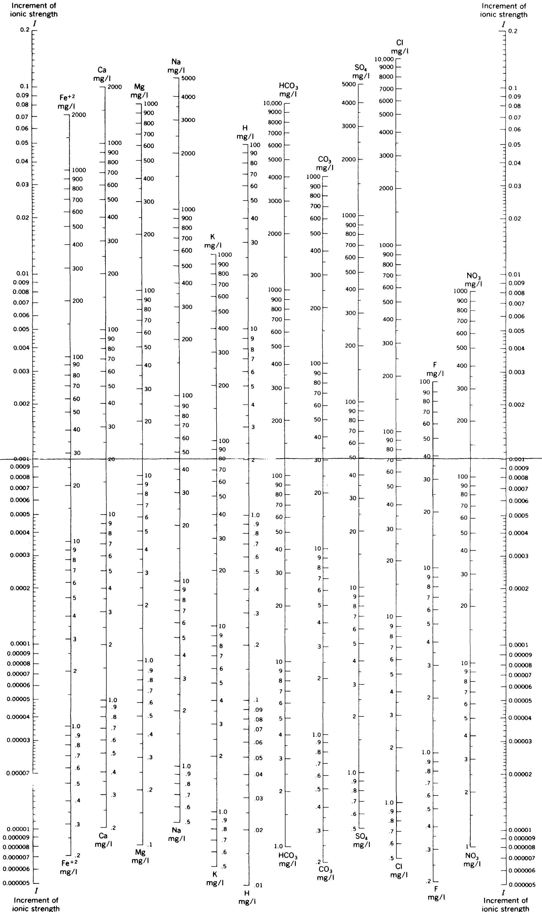
NOMOGRAPH FOR COMPUTING IONIC STRENGTH OF NATURAL WATER
