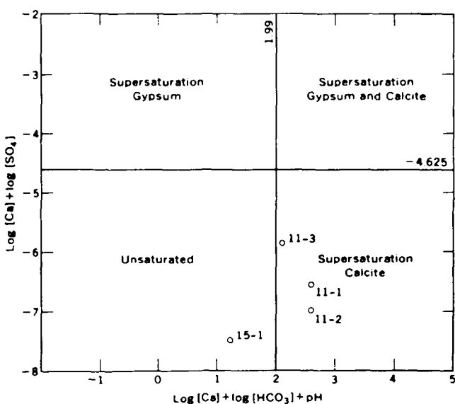
Figure 27. Calcite and gypsum equilibrium solubility relationships, 25°C and 1 atmosphere pressure. Plotted points represent analytical data from tables 11 and 15 (e.g., "11-1"=table 11, analysis 1).
