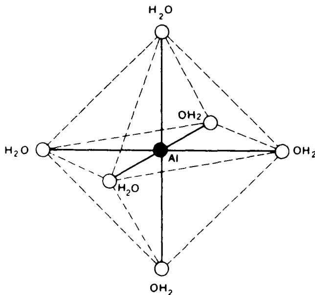
Figure 12. Schematic diagram of hydrated aluminum ion, Al(H_2O)_6^{3+} . (From Hem, 1968b, in "Trace Inorganics in Water," Advances in Chemistry Series, 73, copyright American Chemical Society, 1968, used by permission.)
