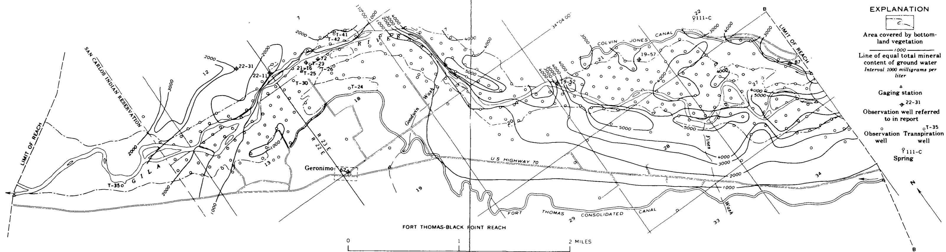
MAP OF PART OF LOWER SAFFORD VALLEY, ARIZONA, SHOWING DISSOLVED-MINERAL CONTENT OF GROUND WATER IN ALLUVIAL FILL OF THE INNER VALLEY, 1944 (GATEWOOD AND OTHERS, 1950)
