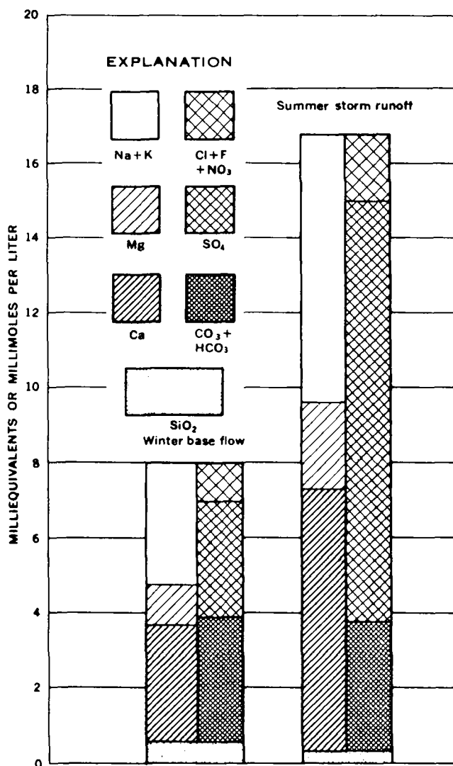
Figure 47. Average composition of water from Rio Grande during two periods in 1945 and 1946.
