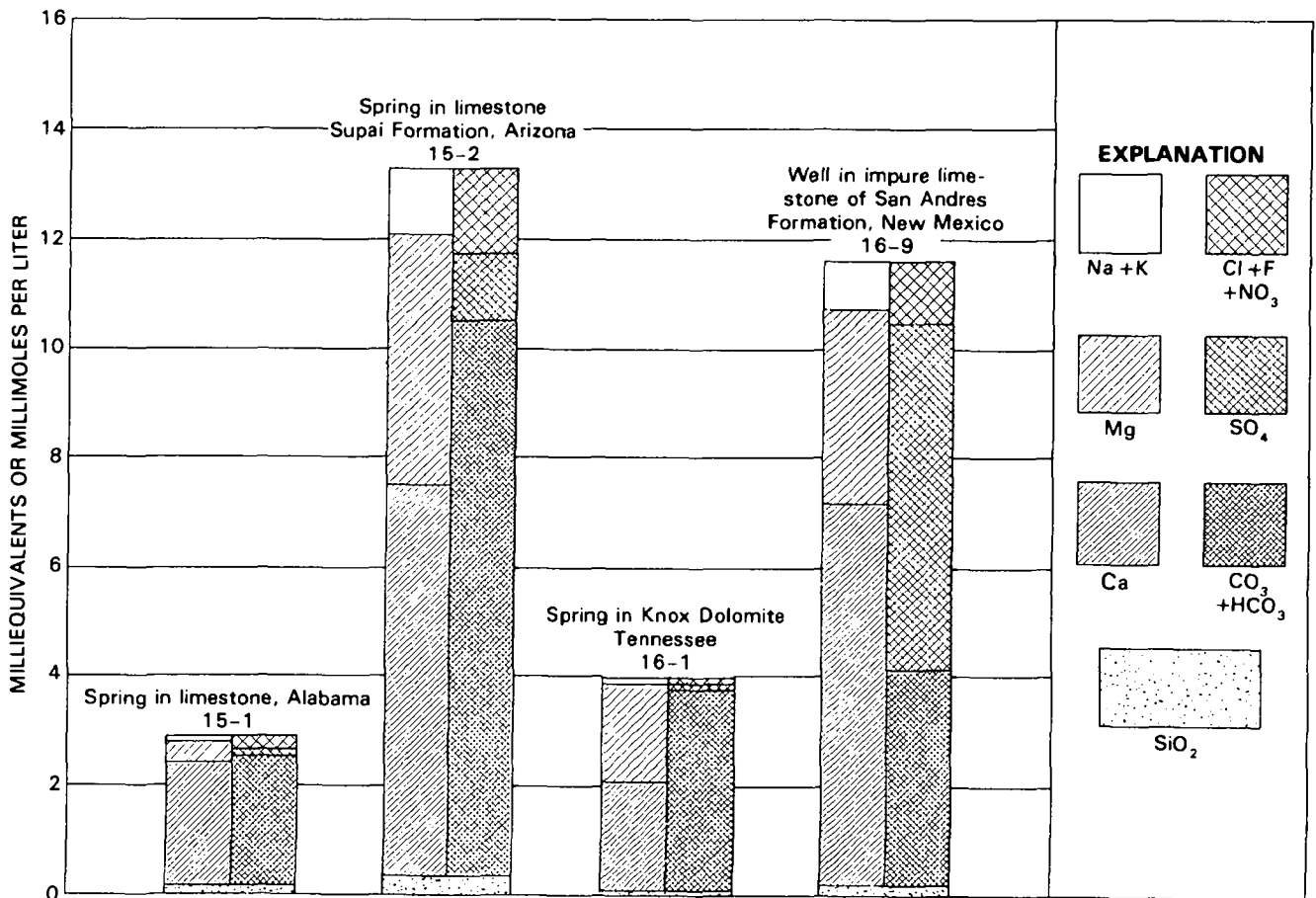
Figure 48. Composition of ground water obtained from precipitate sedimentary rock types. Numbers above bars indicate source of data in tables 15 and 16 (e.g., "15-1"=table 15, analysis 1).
