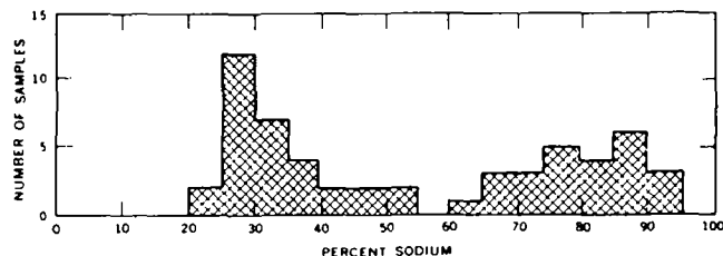
Figure 25. Number of water samples having percent-sodium values within ranges indicated, San Simon artesian basin, Arizona.
