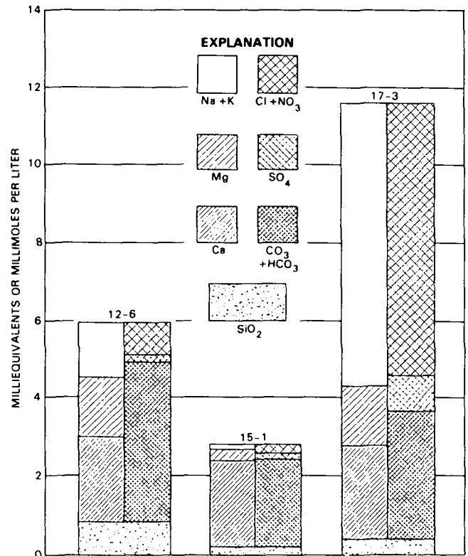
Figure 30. Analyses represented by bar lengths in milliequivalents per liter, with dissolved silica in millimoles per liter. Numbers above bars indicate source of data in tables 12, 15, and 17 (e.g., "12-6"=table 12, analysis 6).
