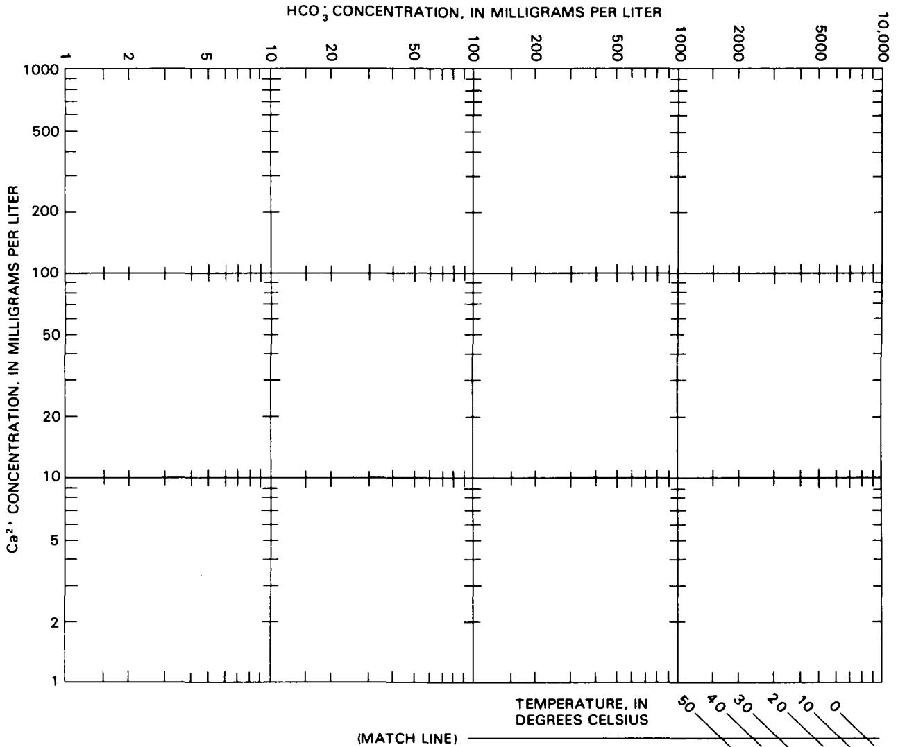
NOMOGRAPH FOR EVALUATING CALCITE EQUILIBRIA - BASE
