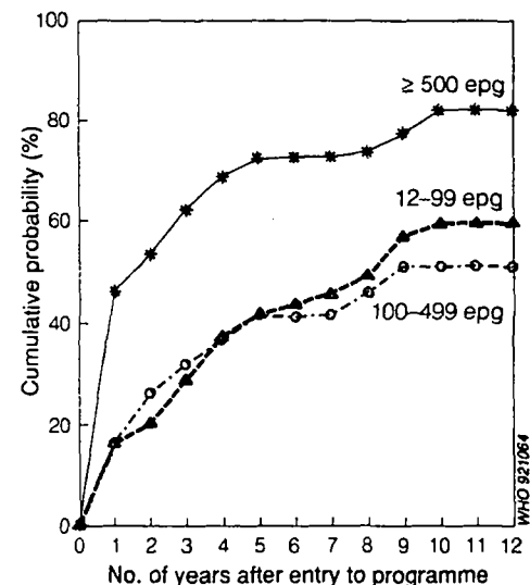
Fig. 1. Cumulative incidence of Schistosoma mansoni reinfection at various years after entry to the programme, according to the number of eggs before treatment (12-99 epg, 100-499 epg and ≥500 epg). These failure estimates are based on data provided by all 296 subjects in the reinfection cohort. The differences over strata were statistically significant ( P < 0.001 in both Wilcoxon and log-rank tests).
