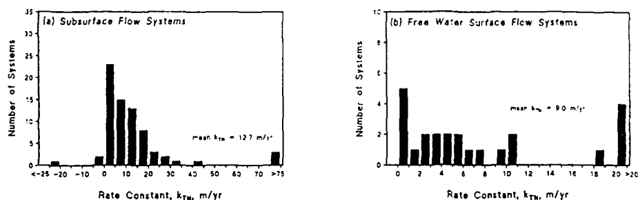
Fig. 9. Frequency distribution of removal rate constants for total nitrogen in (a) subsurface flow ( n=72 ), and (b) free water surface flow ( n=24 ) constructed wetlands
