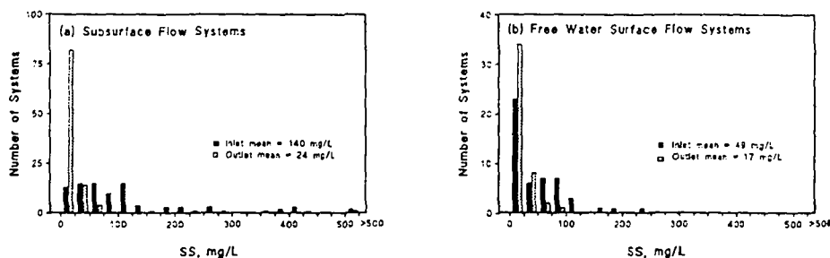
Fig. 3. Frequency distribution of inlet and outlet concentrations of SS in (a) subsurface flow (n=101), and (b) free water surface flow (n=49) constructed wetlands
