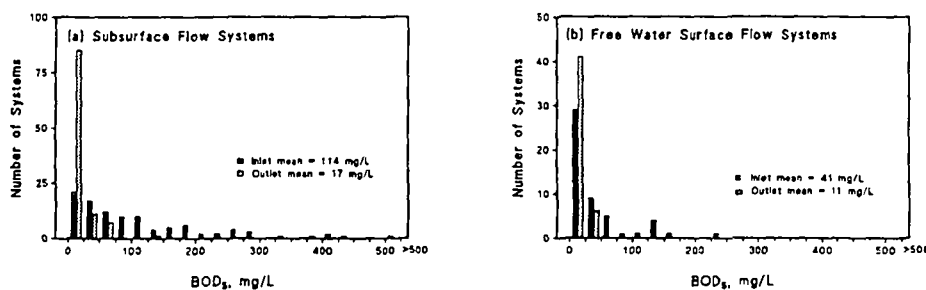
Fig. 4. Frequency distribution of inlet and outlet concentrations of BOD 5 in (a) subsurface flow (n=89), and (b) free water surface flow (n=51) constructed wetlands
