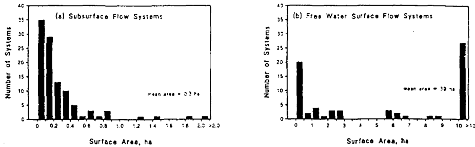
Fig. 1. Size distributions of (a) subsurface flow (n=104), and (b) free water surface flow (n=68) constructed wetlands
