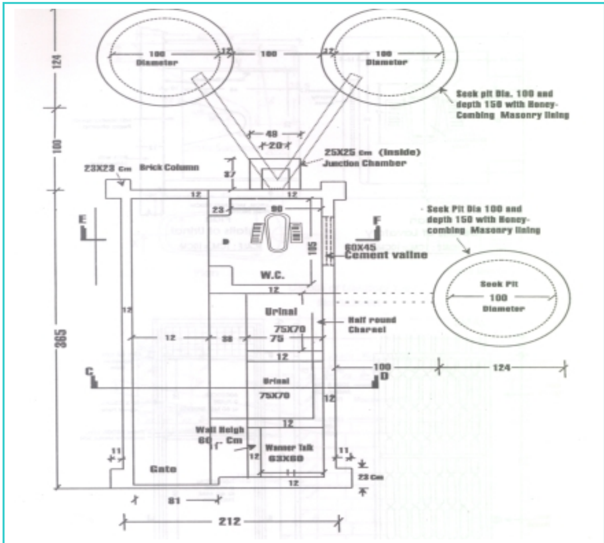
Figure 8- Plan for Urinal and Lavatory for 150 students (especially for girls)
