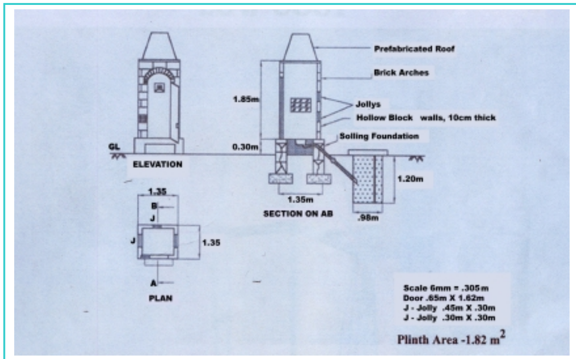
Anganwadi Toilet Design Option 1- Part B
