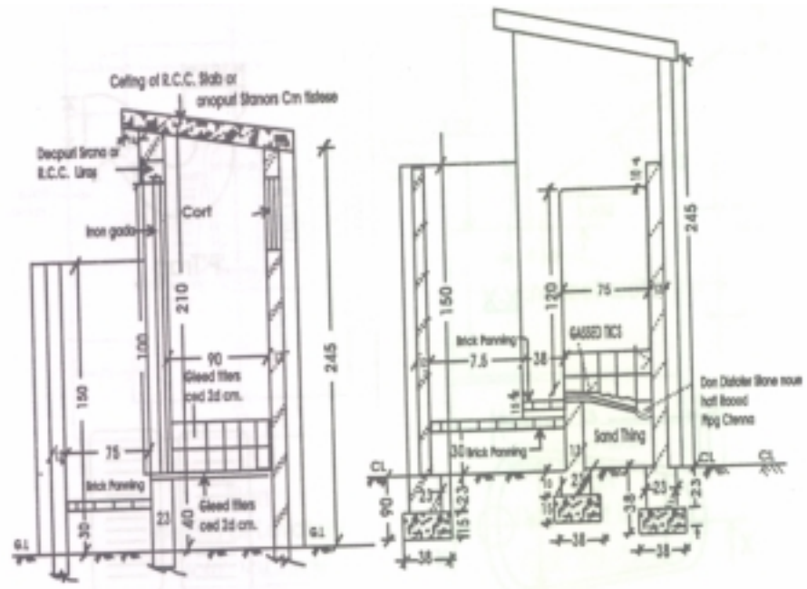
DETAILS OF LAVATORY : CROSS SECTION On E-F DETAILS OF URINAL : CROSS SECTION ON C-D
