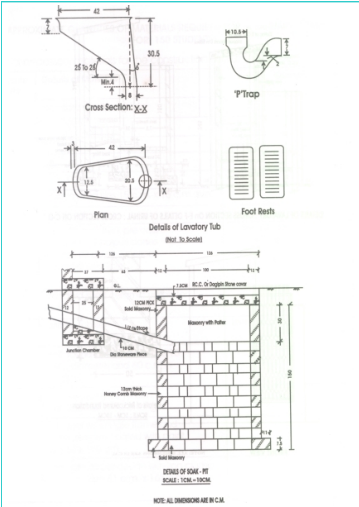
Figure-11 Detail Plan of Pan and Lavatory Tube
