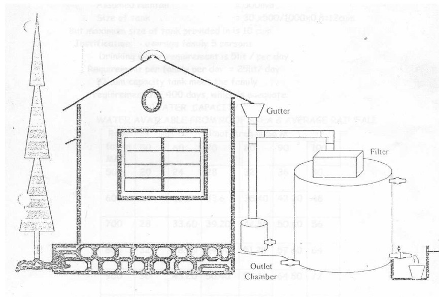
Roof Top Rain Water Harvesting (Direct Collection)
