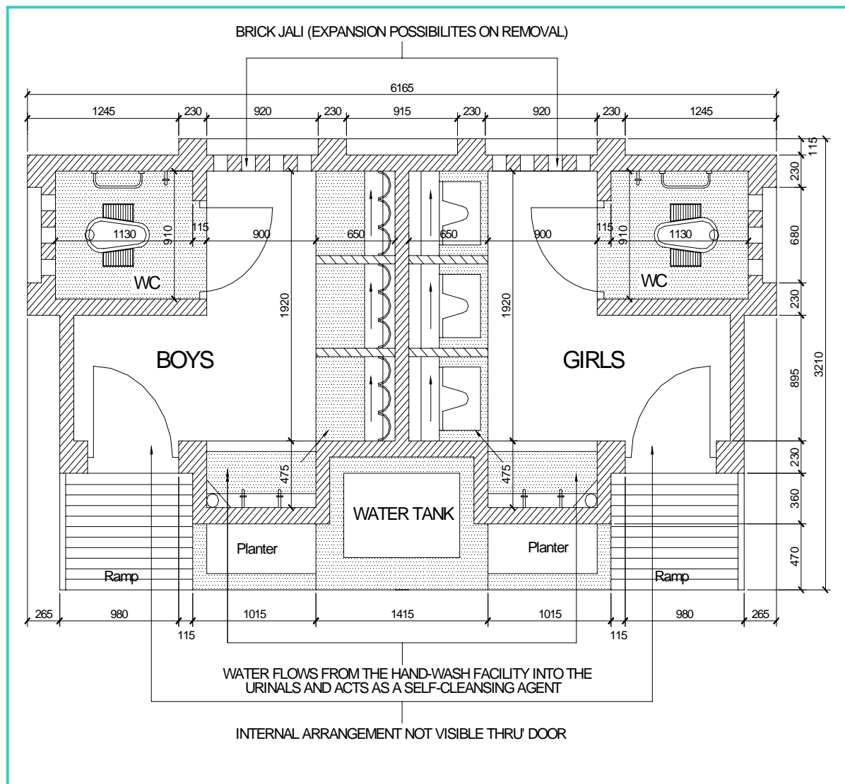
School Toilet Design Option 6 Figure 24- Type- 2
