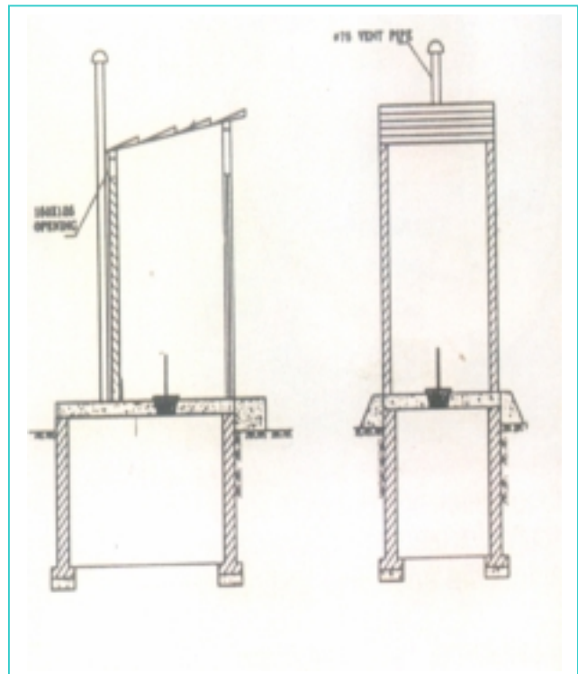
Ventilated Improved Pit Latrine(VIP) Figure 4
