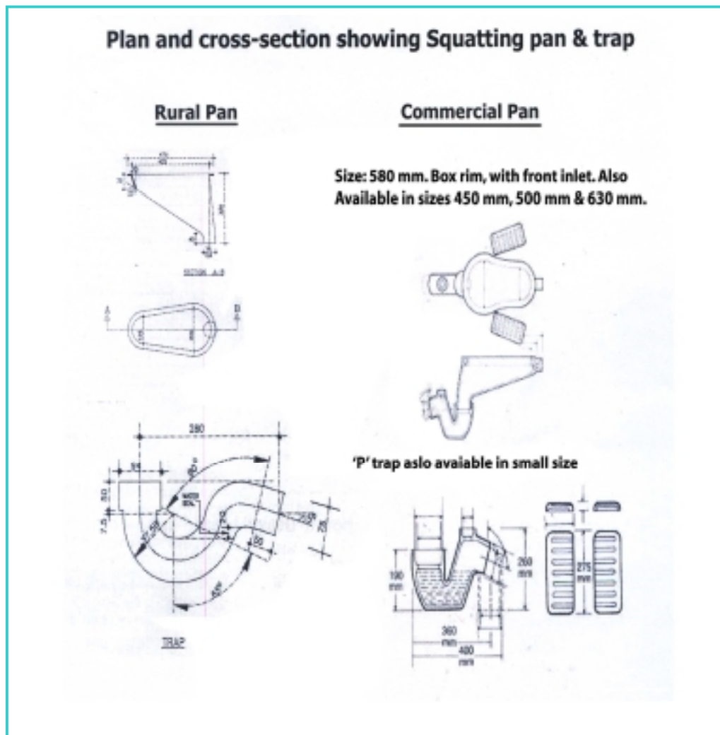
Figure 25- Rural and Commercial Pan Design
