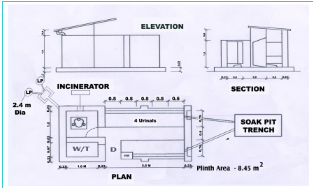
Figure 13- Plan and Cross Section
