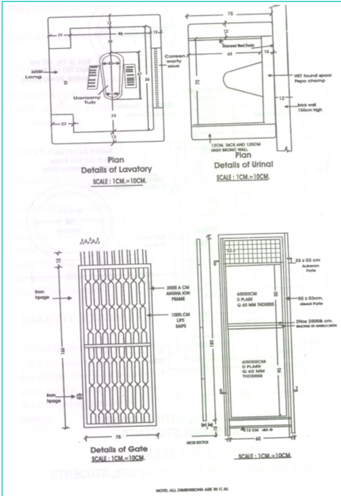
Figure 10- Detail Plan of urinal, lavatory and gate
