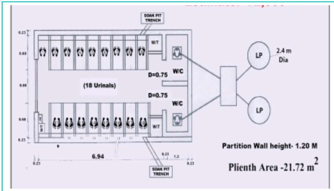
Figure –21 Plan and Cross Section
