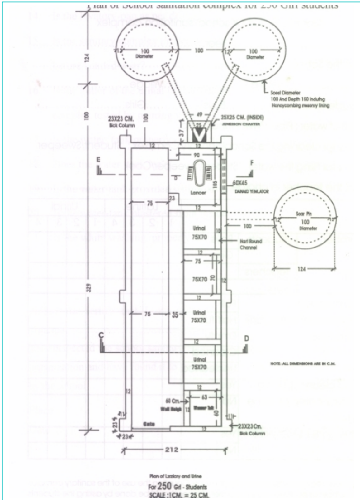
Figure 17- Plan - Type-3
