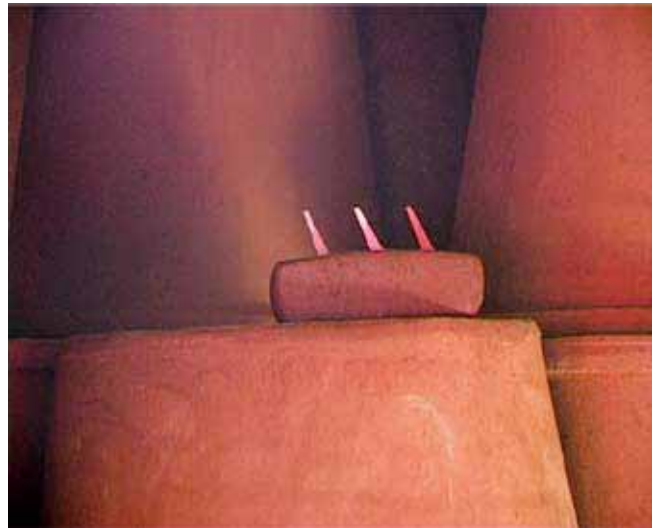
Three cones are used to control the firing temperature – melting at 866°C, 887°C and 950°C.
