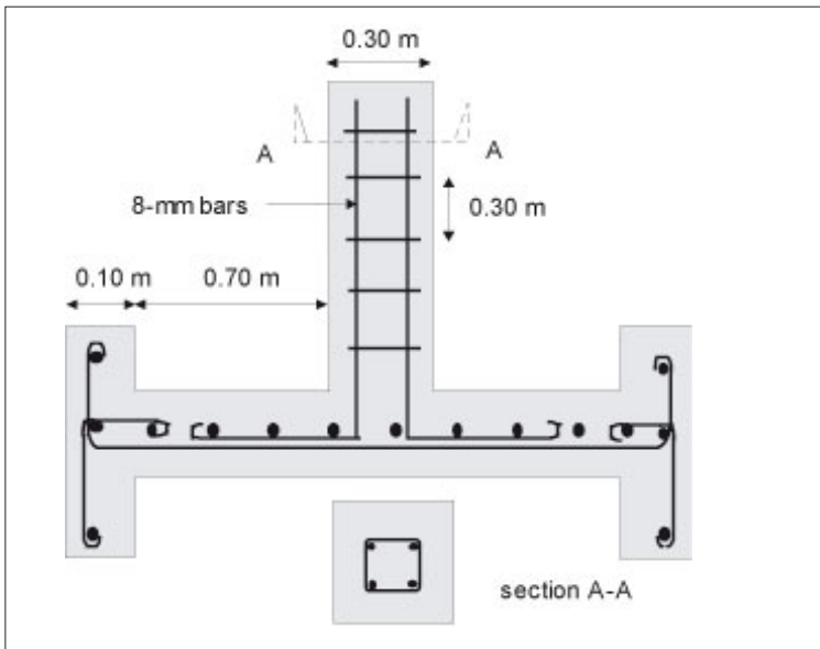
Figure 30: Reinforcement for tapstand and apron.
