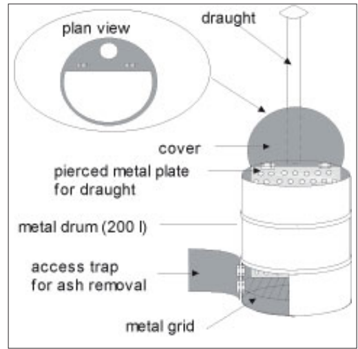
Figure 13.29: Simple incinerator.
