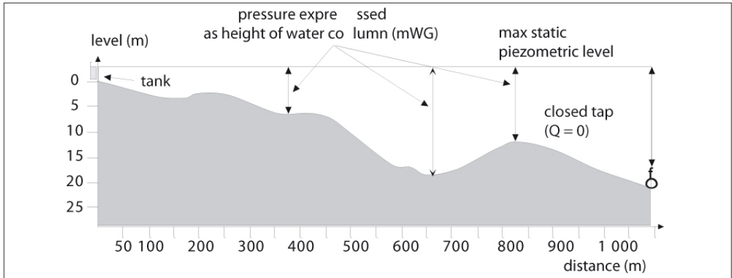
Figure 11.6: Static pressure in a pipe system.
