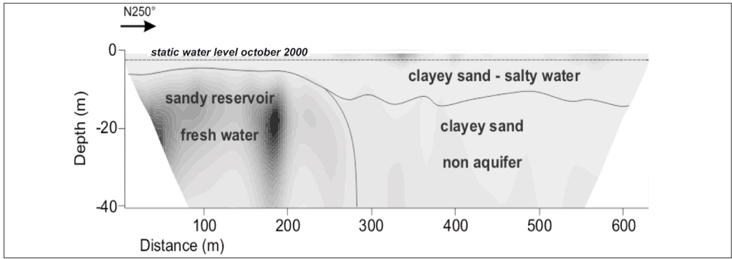
Figure 5.63: Representation of the Chivulivuli aquifer (Mozambique, 2000).
