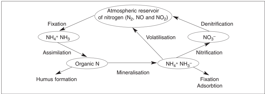
Figure 4.5: The nitrogen cycle.
