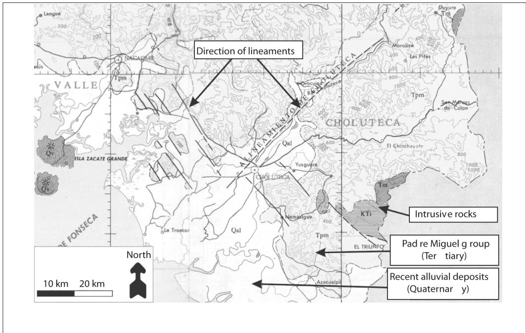
Figure 5.1: Geological map of southern Honduras.
