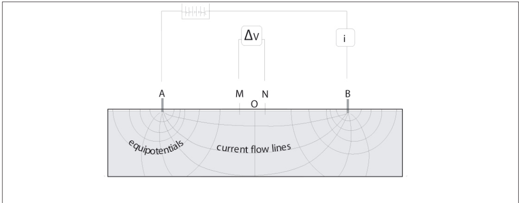
Figure 5.5: Principles of geophysical electrical measurements.
