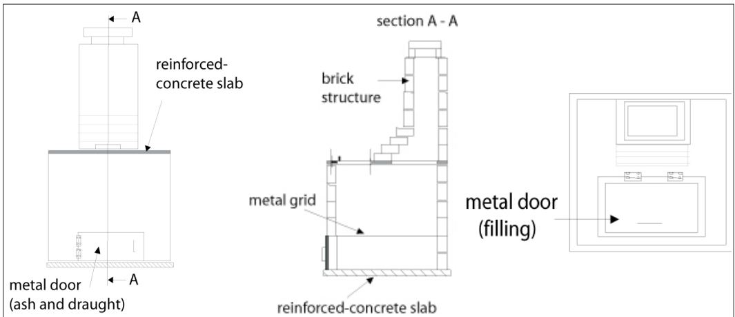
Figure 13.30: Brick-built incinerator.
