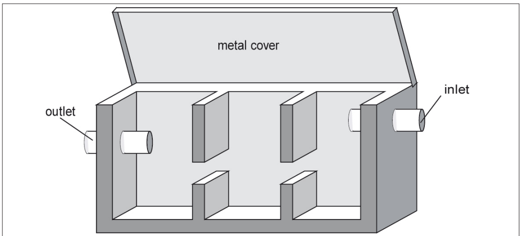
Figure 13.26: Grease trap, ACF Ingushetia 2003.
