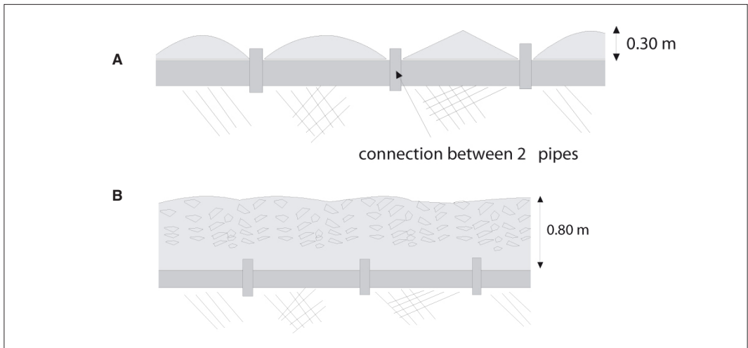
Figure 11.26: Backfilling the pipe trench.
