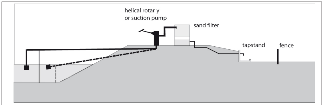
Figure 19.5: Filtration system.
