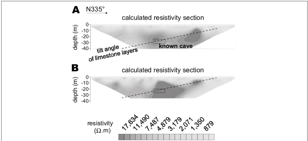
Figure 5.87: ERI interpretation. A: Wenner array. B: dipole-dipole (Wenner beta).
