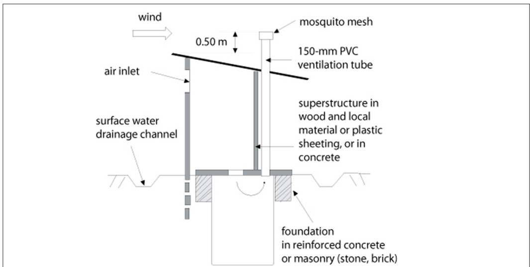
Figure 13.3: Ventilated Improved Pit (VIP).
