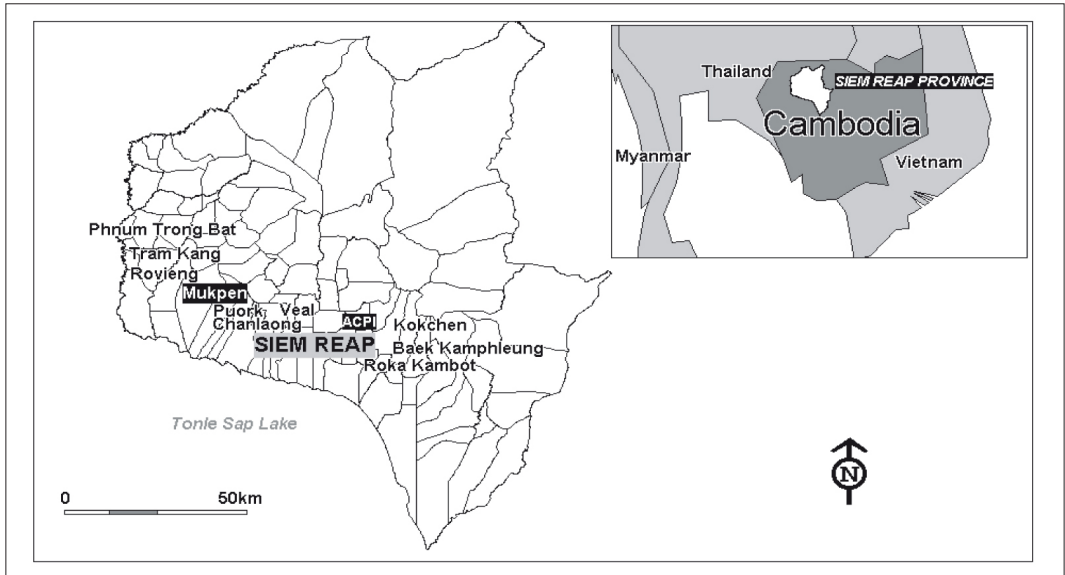
Figure 5.65: Siem Reap Province and main investigated site.
