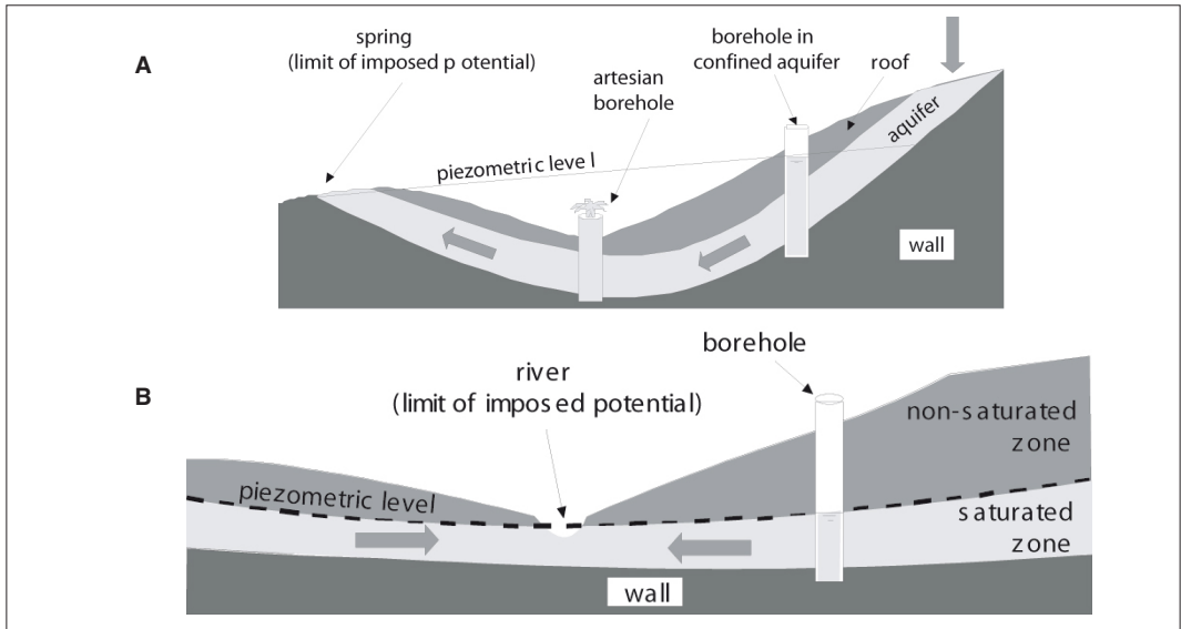
Figure 3.13: Aquifers.
