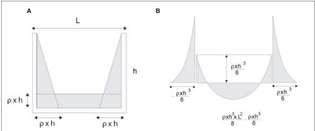
Figure 36: Rectangular tank subject to water pressure. A: diagram of forces (pressure) resulting from weight of water in the tank. B: bending moment diagram in a vertical section of the wall. h: depth of water (m). \rho : density ( \text{kg/m}^3 ).
