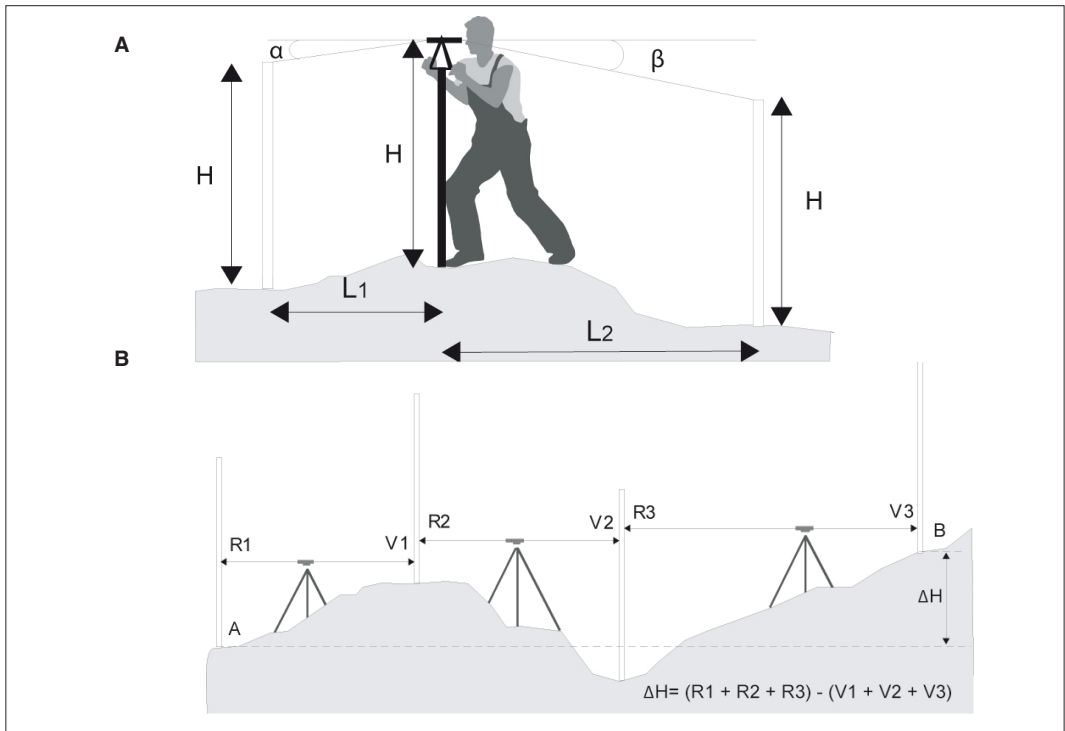
Figure 11.4: Topographic survey.
