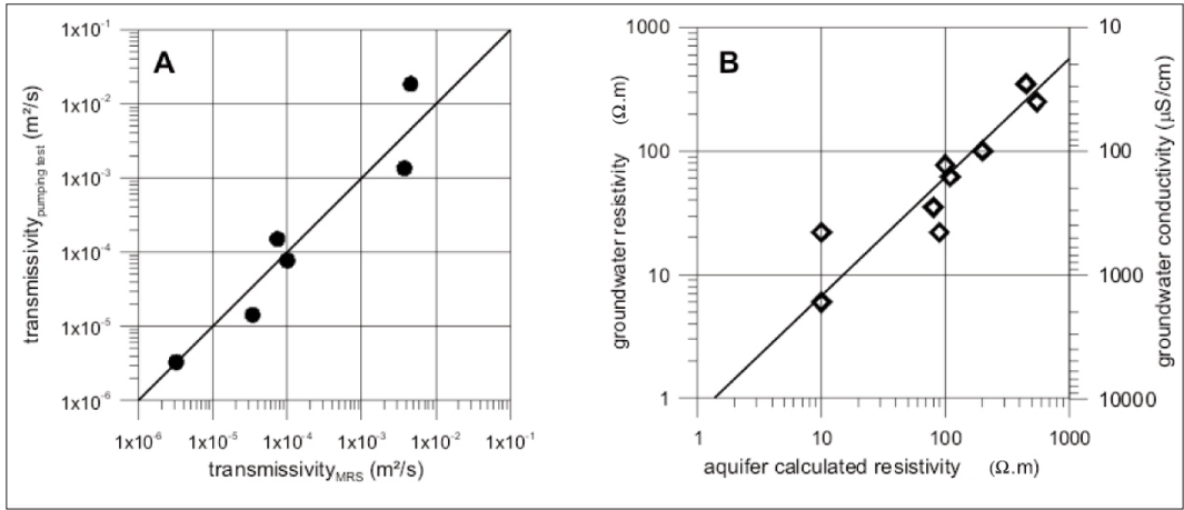
Figure 5.74: MRS hydraulic characterisation. A: local aquifer transmissivity B: groundwater electrical conductivity.
