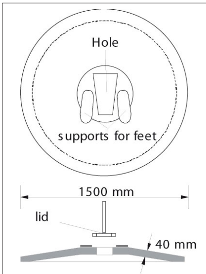
Figure 13.7: Round dome-shaped slab.
