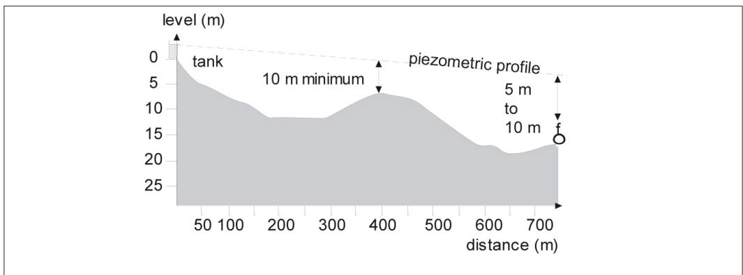
Figure 11.14: Passage over a high point.
