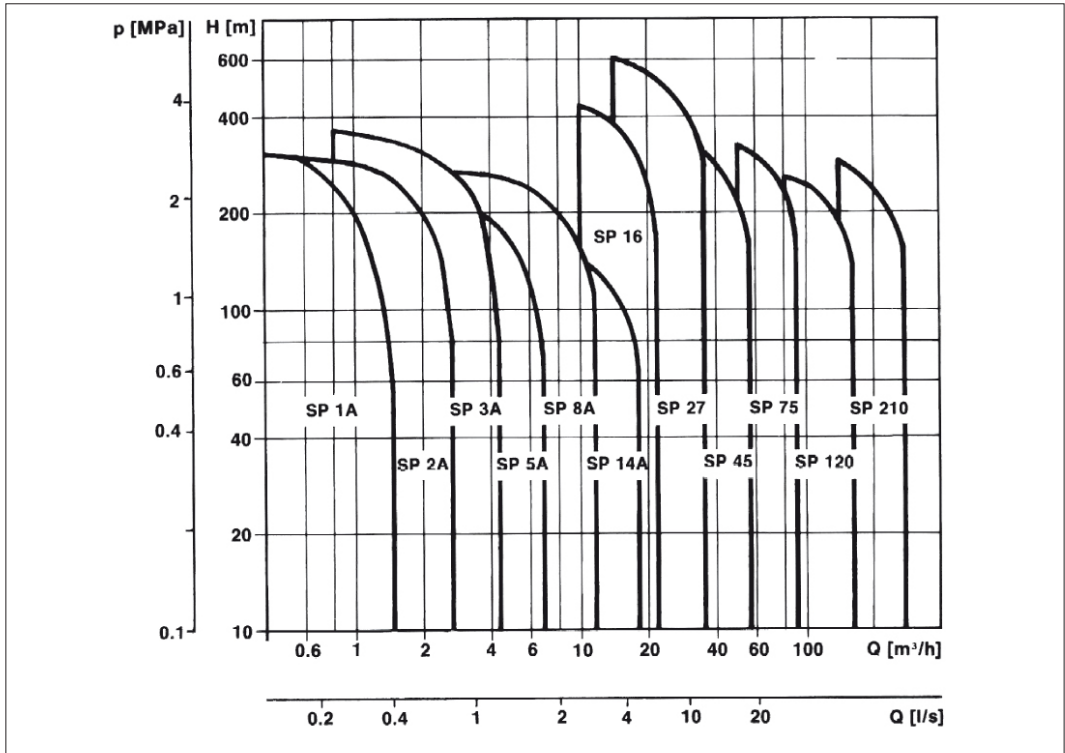
Figure 9.15: Range of Grundfos pumps.
