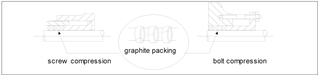
Figure 9.4: Packing.
