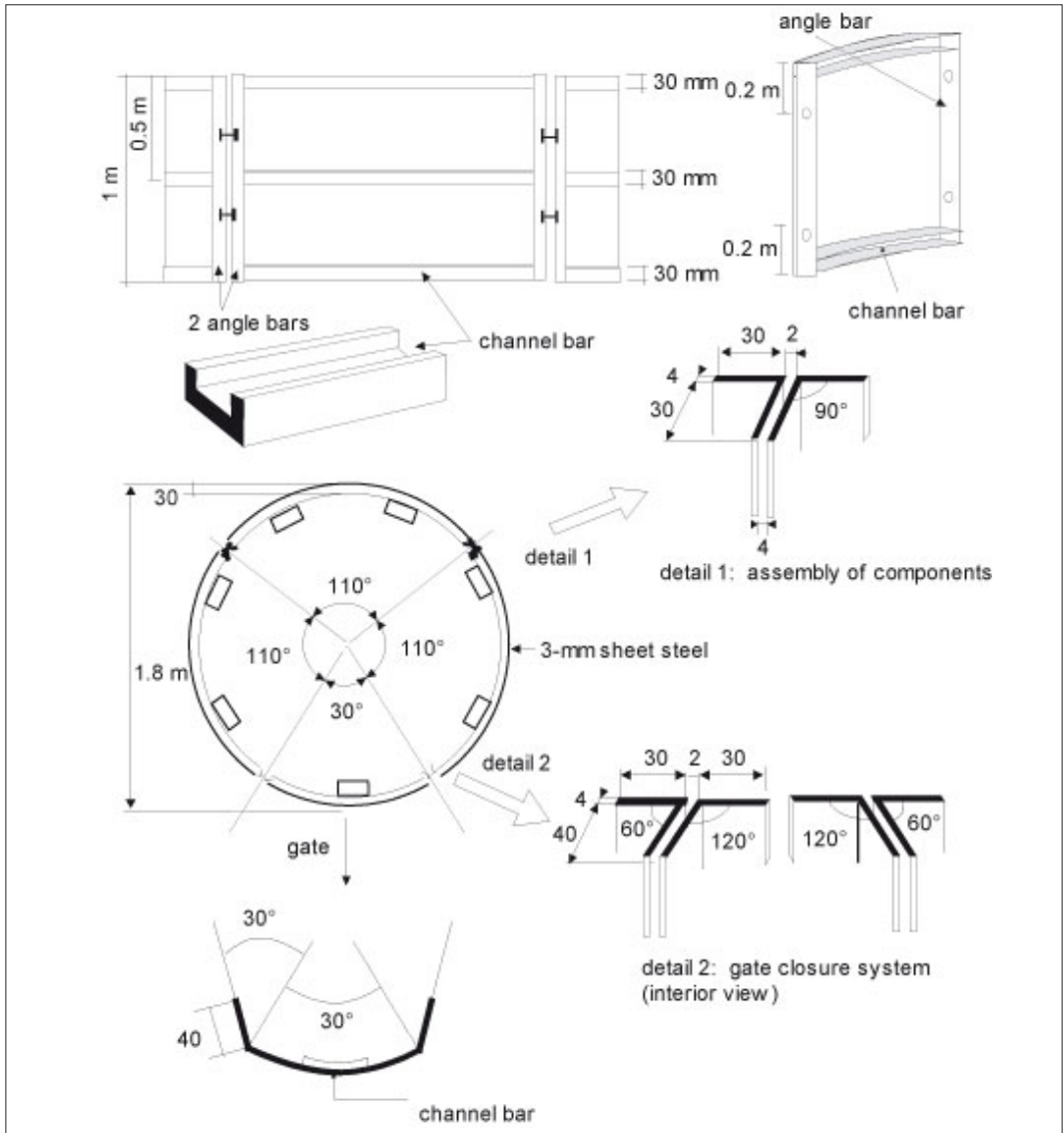
Figure 47: Sliding shuttering for a 1.8-m diameter well.
