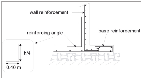
Figure 21: Wall reinforcement for a high-capacity rectangular tank.
