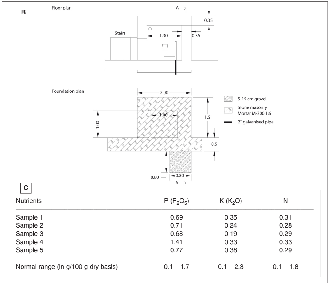
Figure 13.20: Vault latrine (ACF, Afghanistan).
