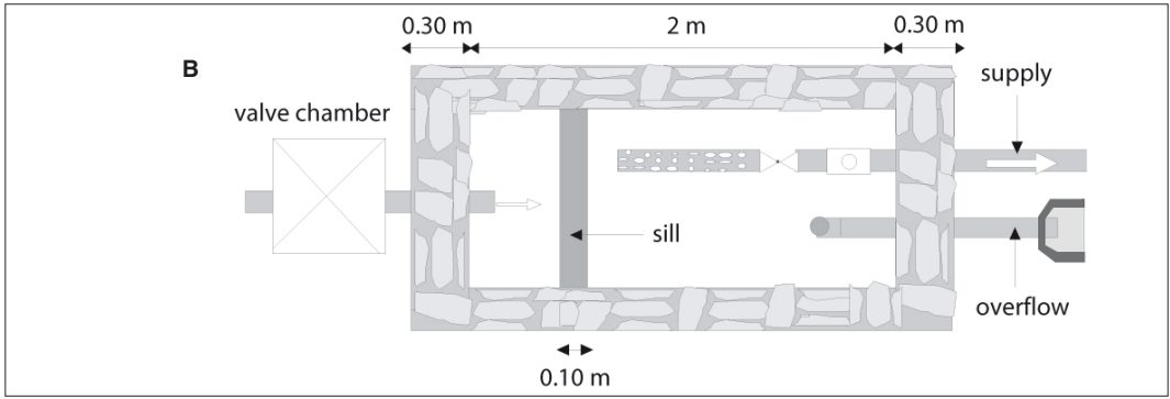
Figure 11.18: Masonry break-pressure tank. B: plan.
