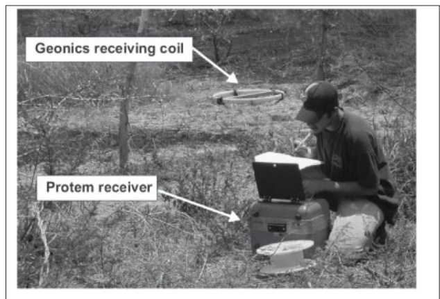
Figure 5.44: Protém equipment (ACF, Honduras, 2000).
