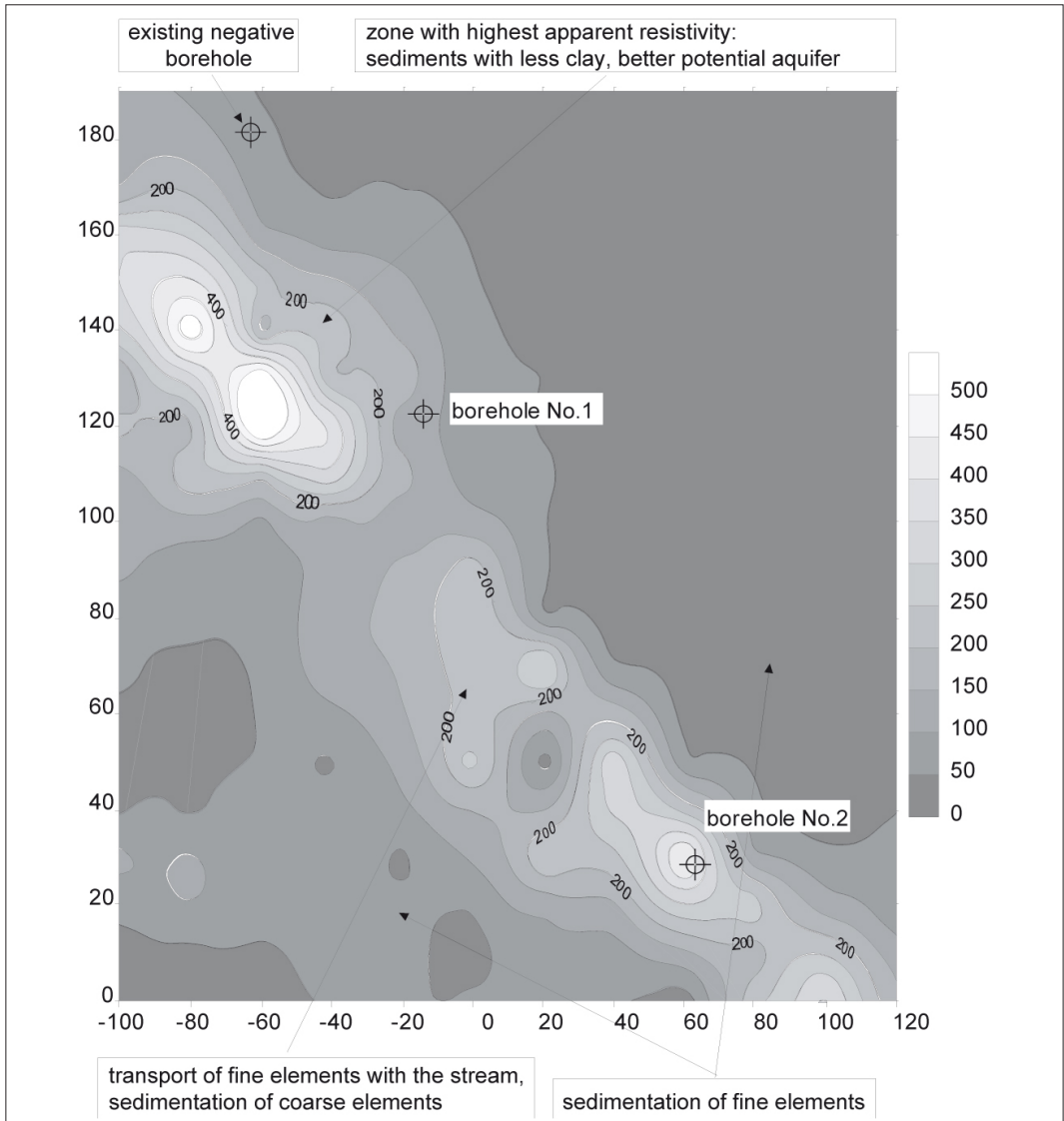
Figure 5.36: Iso-resistivity map (ACF, St André Farm, France, 1995).
