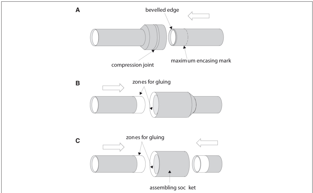
Figure 11.22: PVC pipe joints.
