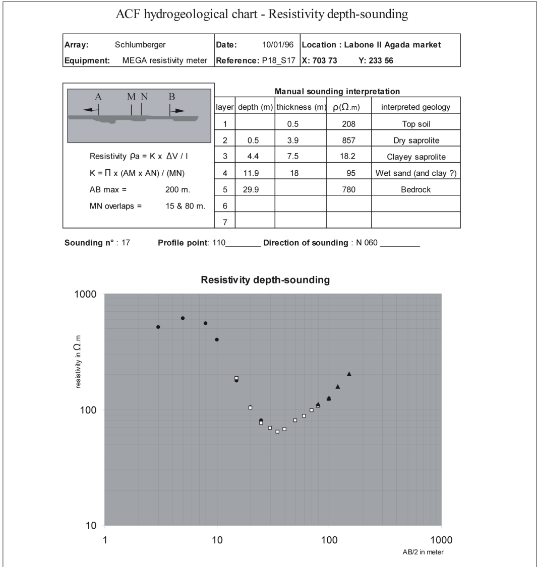
Figure 5.19: Results of VES interpretation (ACF, Sudan, 1996).
