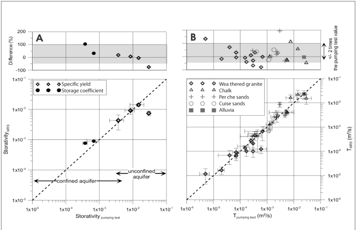
Figure 5.53: MRS hydrogeological estimators. A: storativity estimators for weathered granite in Burkina Faso. B: transmissivity estimator.
