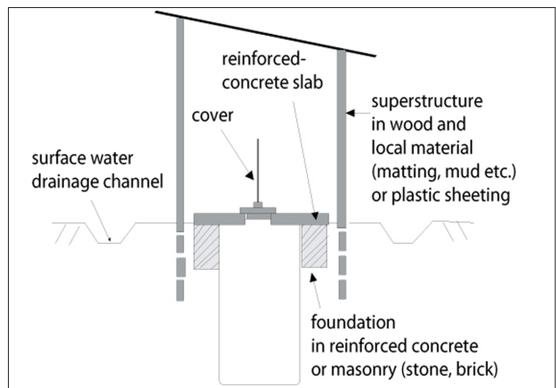
Figure 13.2: Simple pit latrine.
