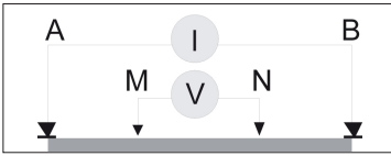
Figure 5.7: Wenner array.
