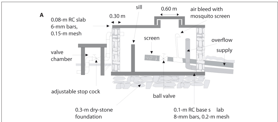
Figure 11.18: Masonry break-pressure tank. A: section.
