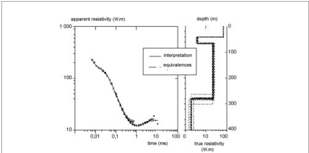
Figure 5.45: Example of TDEM sounding (ACF, Cambodia, 1998).
