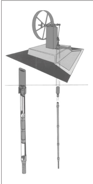
Figure 9.31: Volanta handpump.
