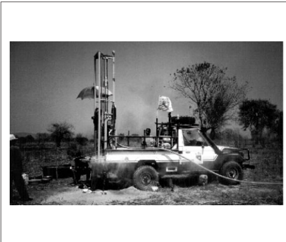
Figure 6: Rig on a vehicle.
