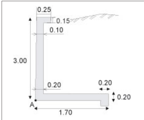
Figure 42: Reinforced-concrete retaining wall.
