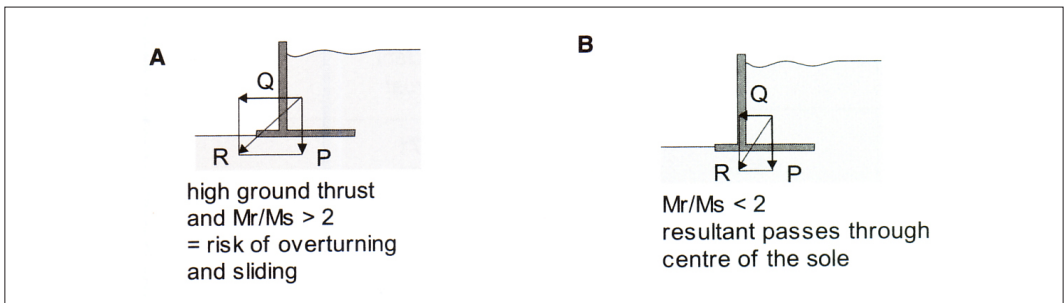
Figure 40: Conditions of non-overturning and non-sliding.
