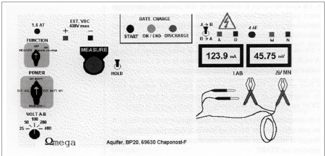
Figure 1: Front of the Omega resistivity meter.
