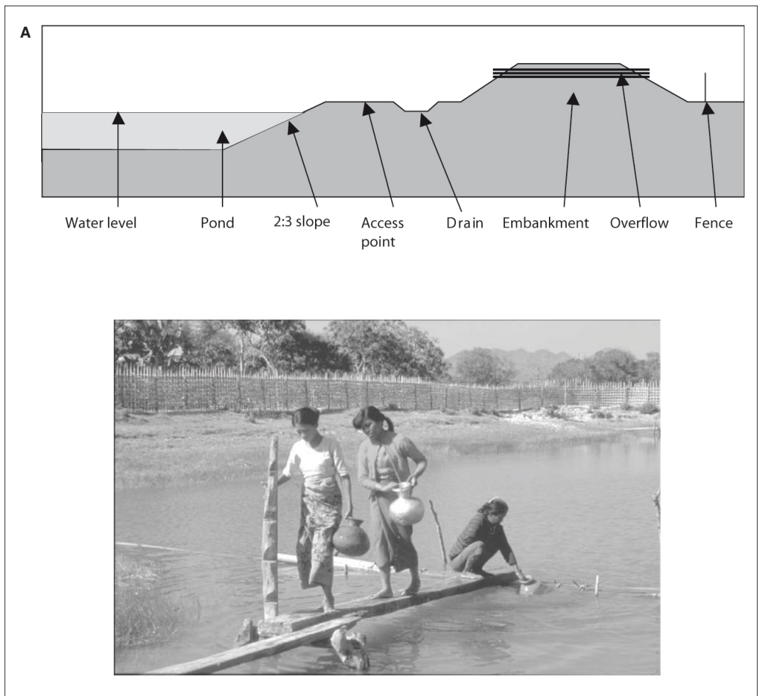
Figure 19.1: Community pond (ACF, Myanmar, 1996). A: construction plan. B: water-collection system.
