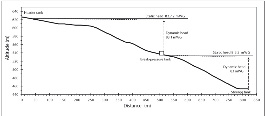
Figure 3: Main supply line.
