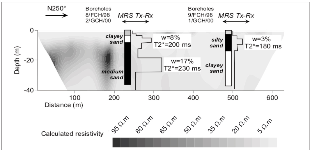
Figure 5.62: ERI and MRS, Chivulivuli Site (Mozambique, 2000). W is the water fraction and T_2^* the measured decay constant.
