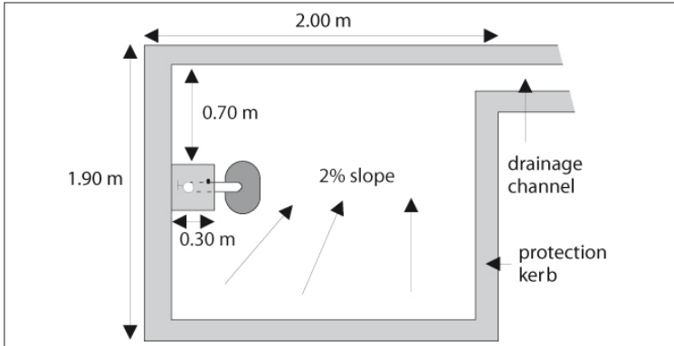
Figure 29: General plan of tapstand and apron.
