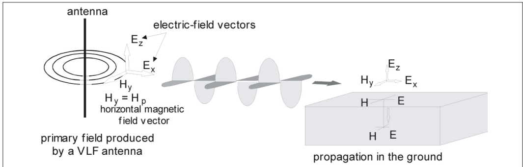
Figure 5.33: Primary electromagnetic field.
