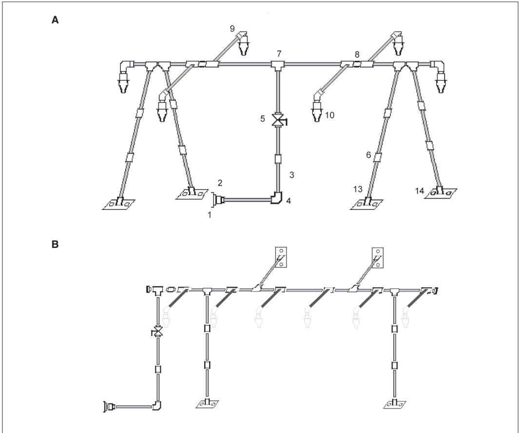
Figure 17.4: ACF tapstand kit. A: standard installation. B: installation against a wall.
