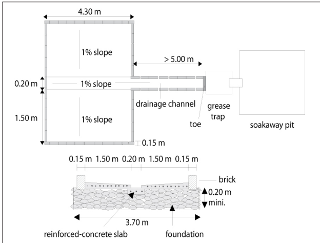
Figure 13.25: Washing area with soakaway pit.
