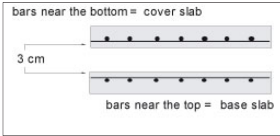
Figure 10: Location of main reinforcement bars according to type of slab (base or cover).
