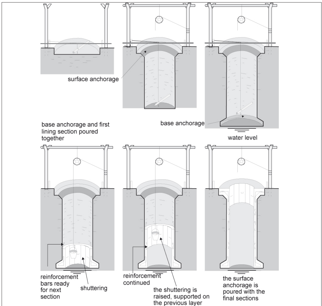
Figure 7.6: Bottom-up lining.
