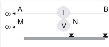
Figure 5.8: Pole-pole array.
