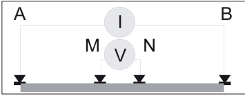
Figure 5.6: Schlumberger array.
