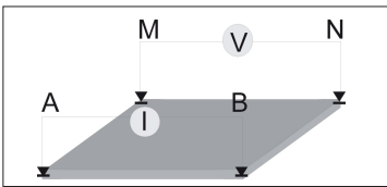
Figure 5.10: Square array.
