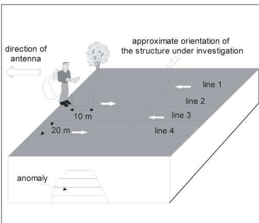
Figure 5.39: TVLF profile in resistivity mode.
