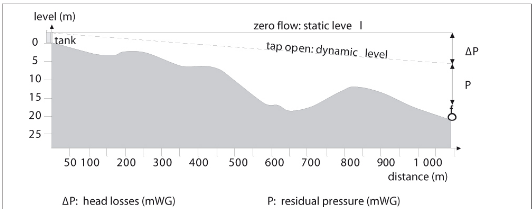
Figure 11.9: Dynamic state and head losses.
