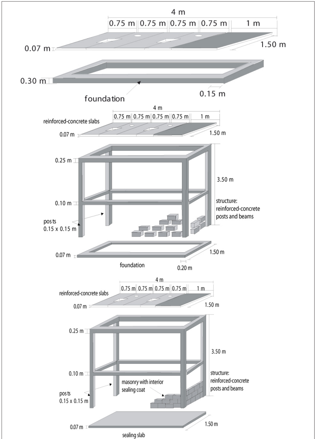
Figure 13.4: Pit and foundation of 2-station latrine.
