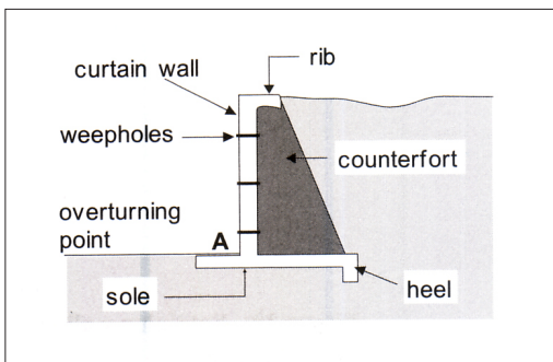
Figure 41: Standard configuration of reinforced-concrete retaining walls.
