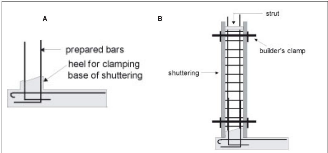
Figure 44: Shuttering for a pillar or curtain wall.
