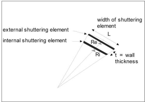
Figure 2: Geometric projection of a shuttering element.
