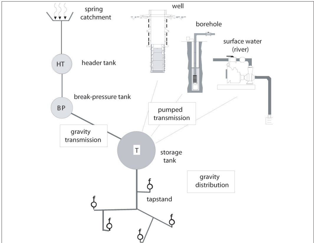
Figure 11.1: Distribution system: various possible schemes.
