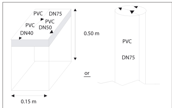
Figure 11.30: Pipe anchors.
