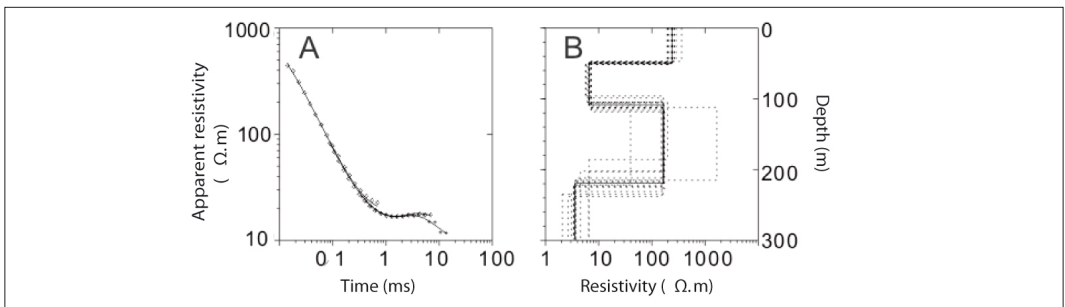
Figure 5.68: TDEM sounding, ACPI school. A: field data. B: inversion (equivalent models, best fit rms error = %).
