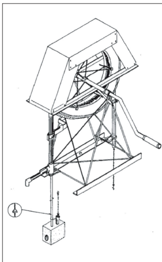
Figure 9.38: Rope pump.
