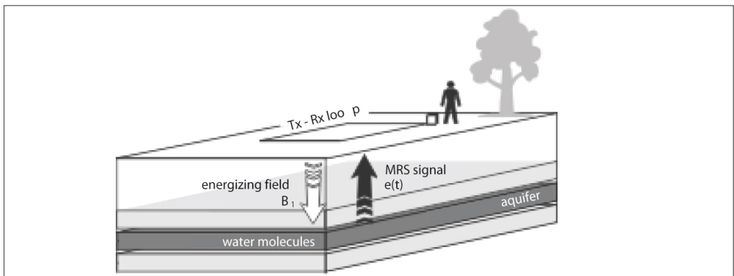
Figure 5.48: Schematic diagram of MRS measurement array.
