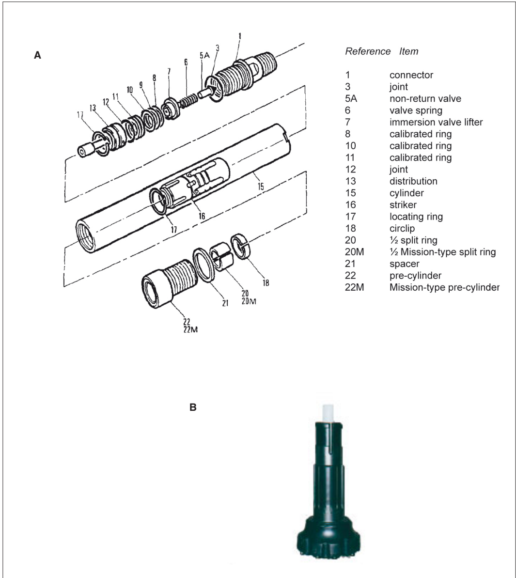
Figure 12: Down-the-hole hammer.
