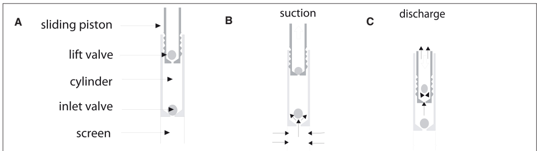
Figure 9.25: Working principle of a piston pump.
