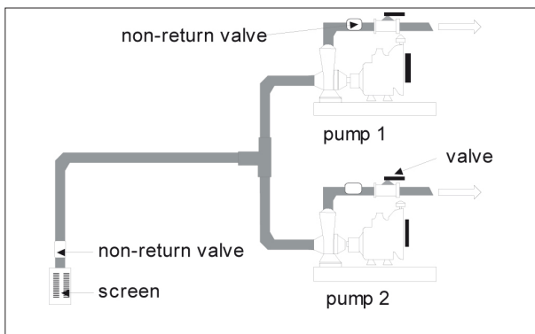
Figure 9.10: Mounting two pumps in parallel.
