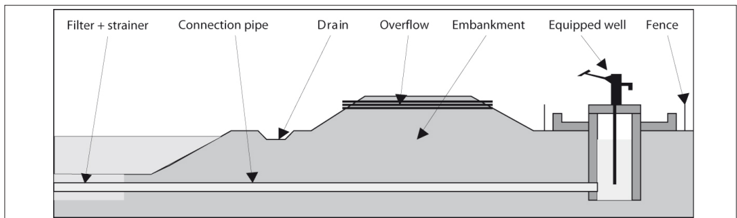
Figure 19.4: Well connected to pond.
