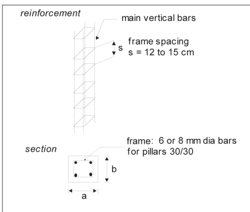
Figure 7: Reinforcement for a pillar.
