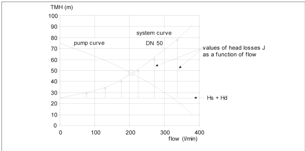
Figure 9.6: Working point (TEF2-50 pump in pipe system).
