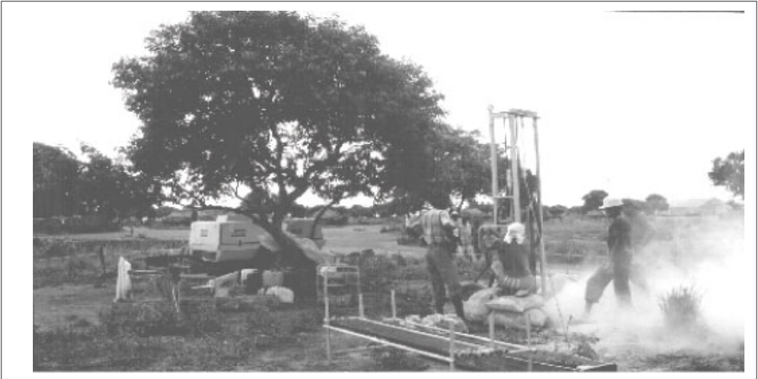
Figure 5: ACF-PAT 301. Rig on the ground.
