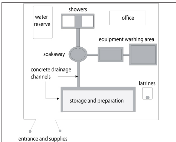
Figure 13.27: Insecticide preparation area.
