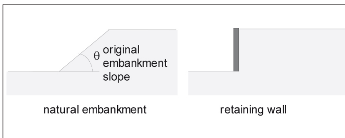
Figure 38: Retaining wall for an embankment.
