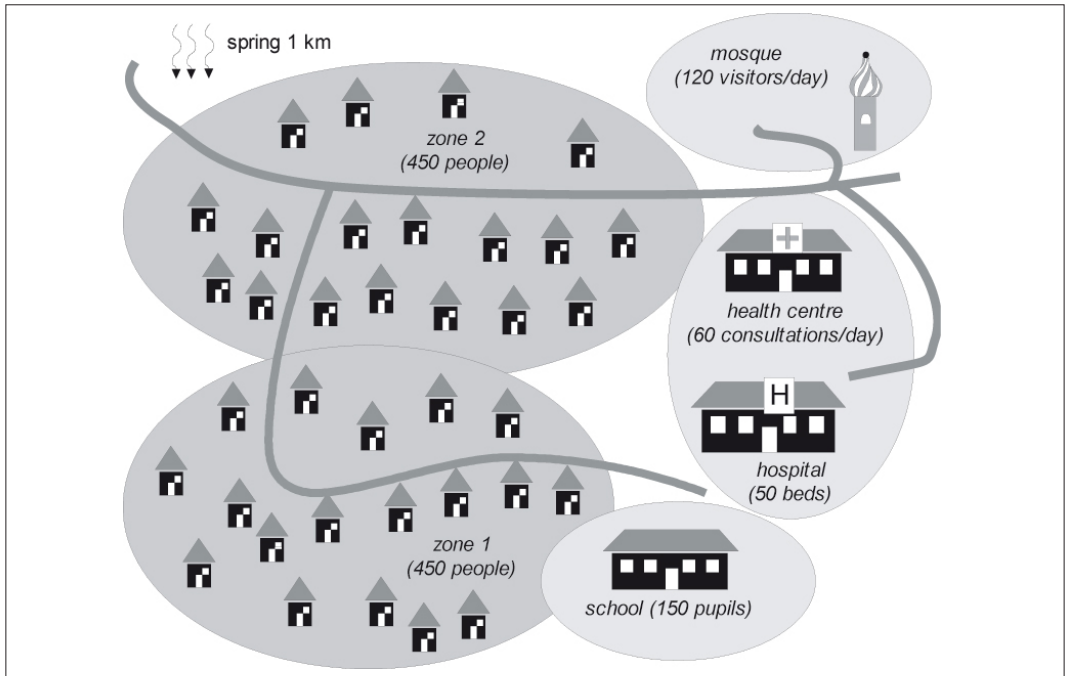
Figure 11.2: Layout plan delimiting distribution zones: Aloua village.
