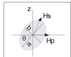
Figure 5.34: Ellipse of polarisation of the field resulting from the interaction between primary and secondary fields.
