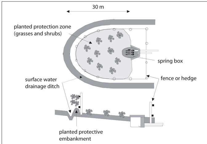
Figure 2: Protection zone of a spring.
