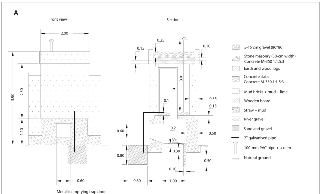
Figure 13.20: Vault latrine (ACF, Afghanistan). A: general design.
