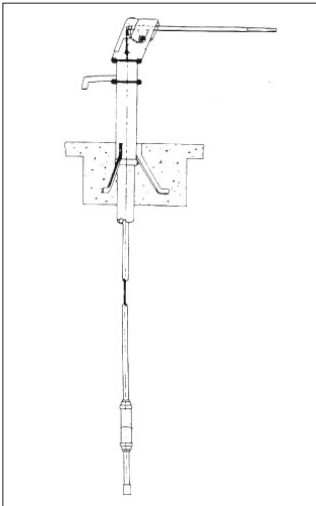
Figure 9.29: India Mark II pumps.
