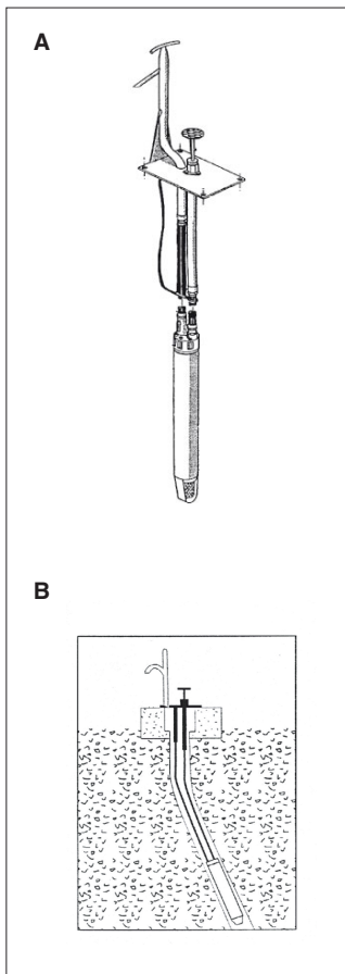
Figure 9.33: Working principle of Vergnet hydropump.
