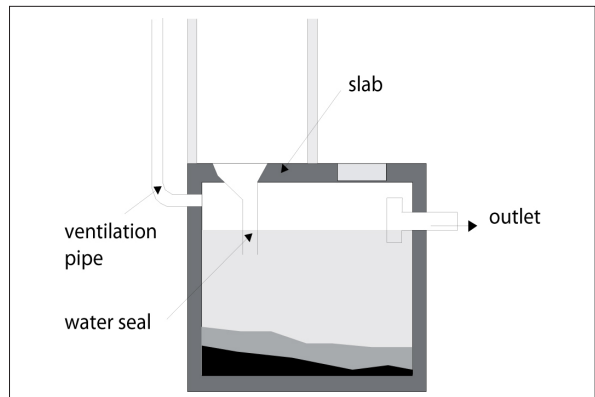
Figure 13.15: Aqua-Privy.
