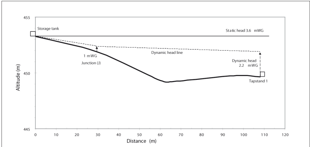
Figure 4: Storage tank to tapstand 1.
