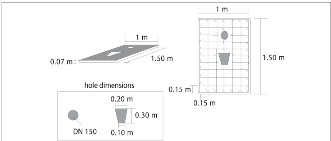
Figure 13.5: Reinforcement for a single slab.
