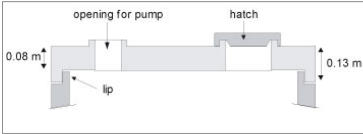
Figure 28: Well cover and inspection hatch.
