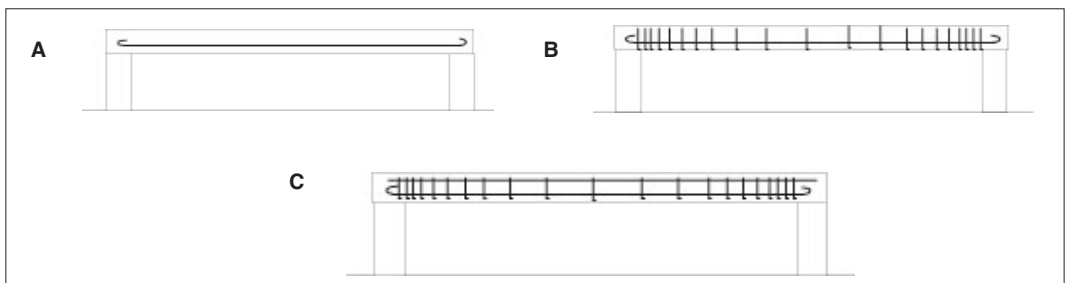
Figure 32: Reinforcement of a beam on free supports.
