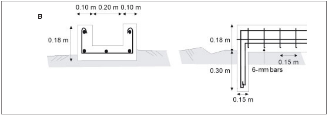
Figure 26: Reinforcement. B: drainage channel.
