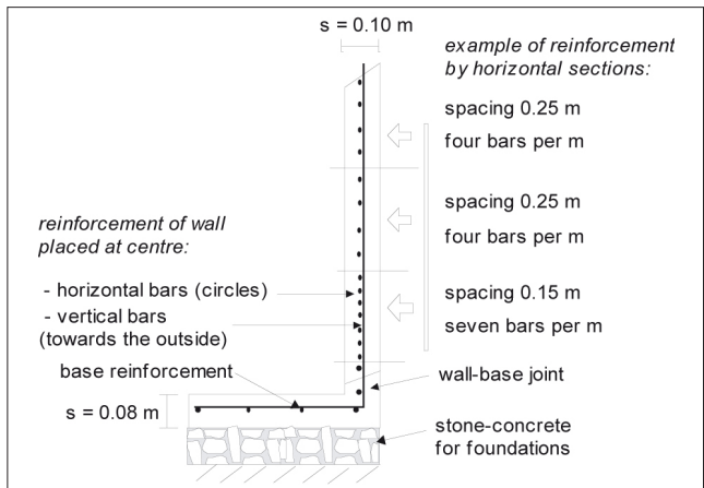
Figure 18: Example of reinforcement for a circular tank.
