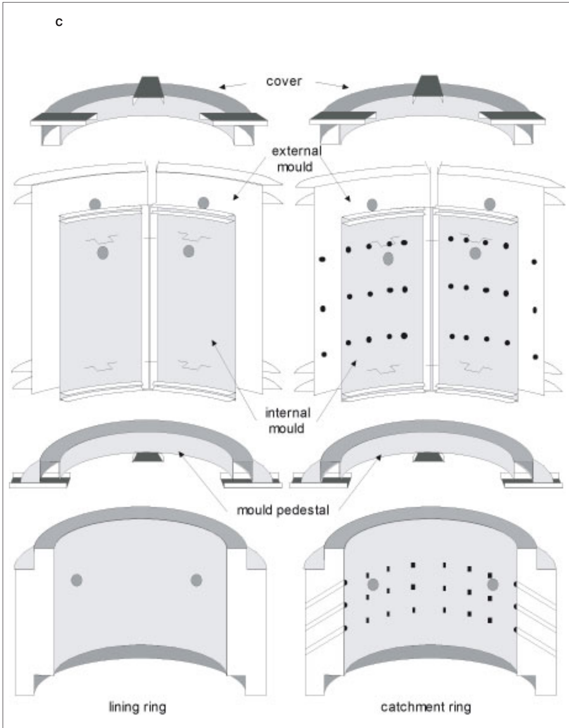
Figure 45: Metal shuttering for a concrete-ring mould.
