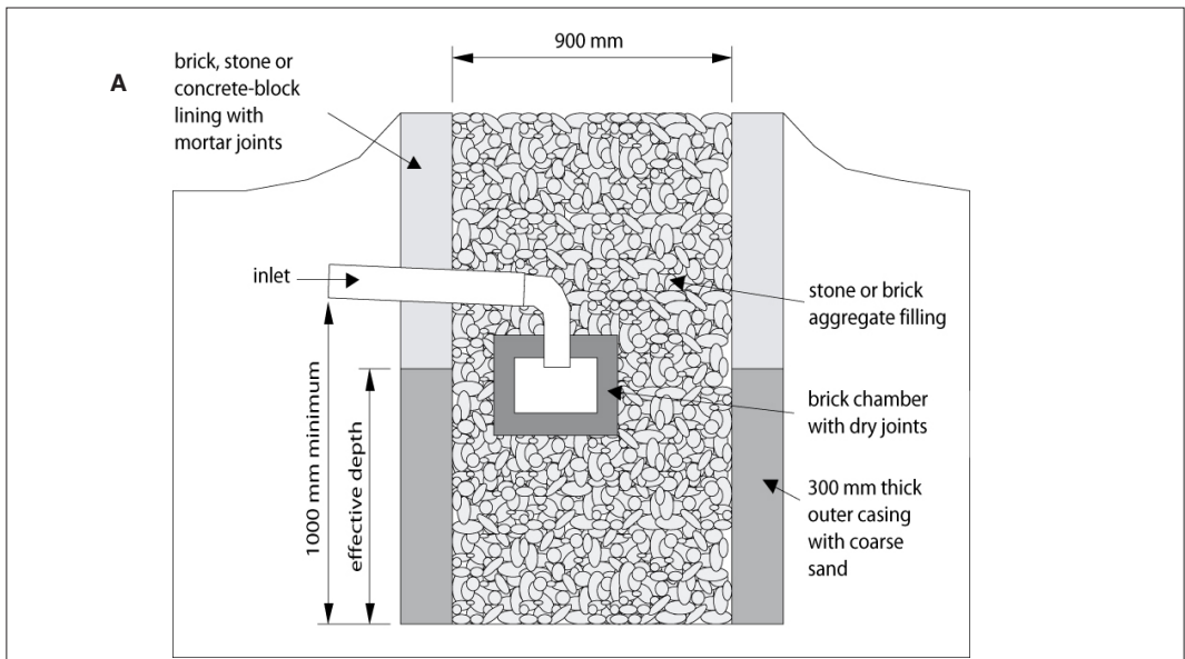
Figure 13.16: Soakaway pits. A: unlined pit.
