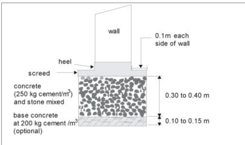
Figure 15: Section through a foundation.
