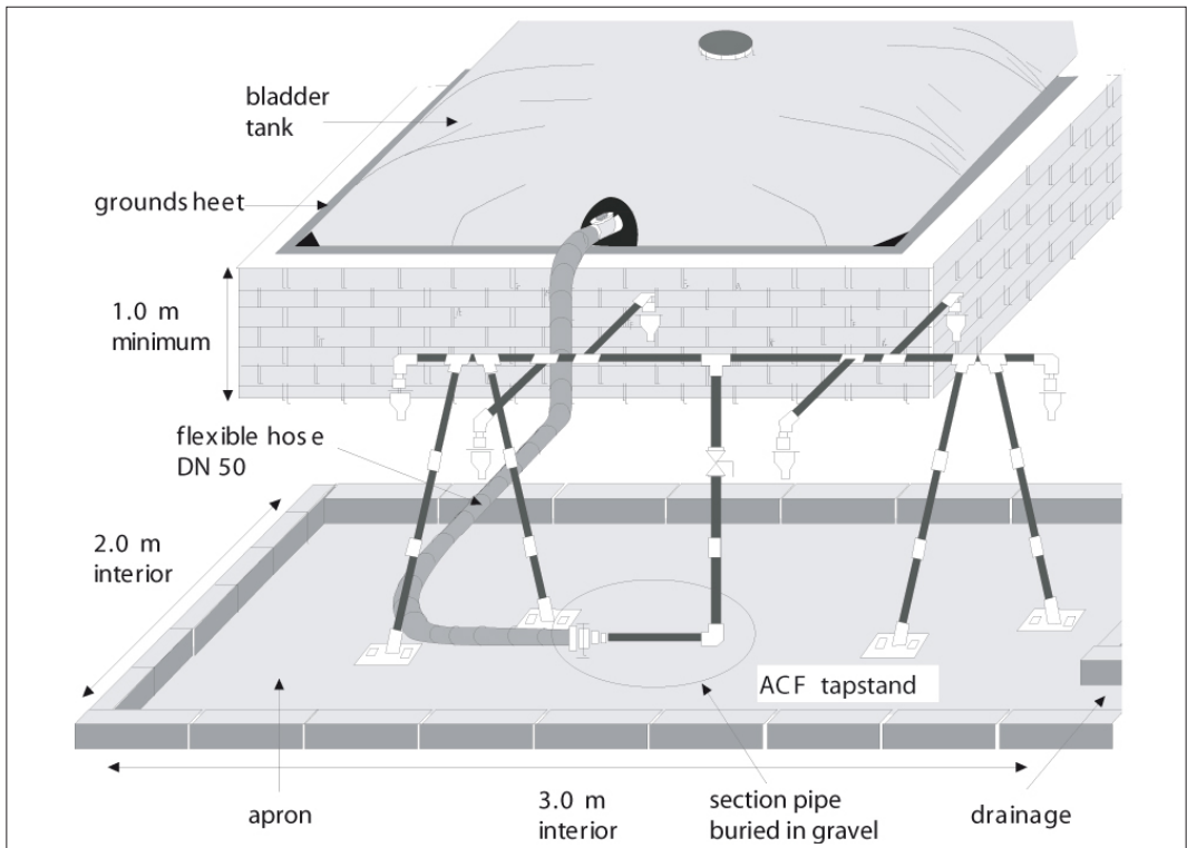
Figure 17.3: Flexible tank (bladder type) and tapstand.
