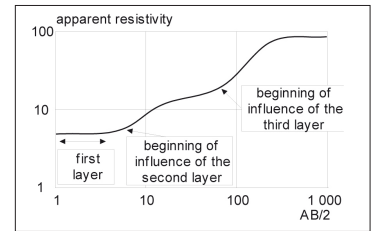
> Figure 5.22: Three-layer curve.
