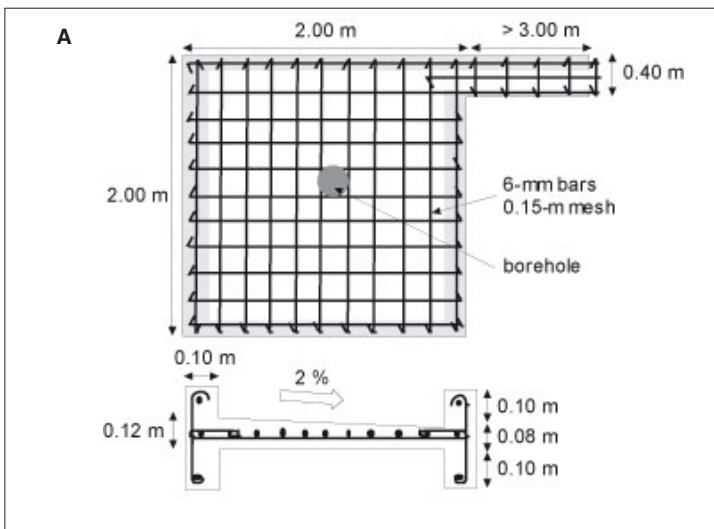
Figure 26: Reinforcement. A: slab.
