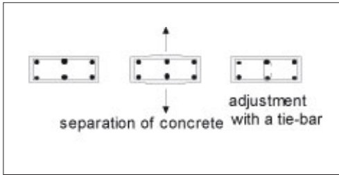
Figure 5: Reinforcement for a pillar.
