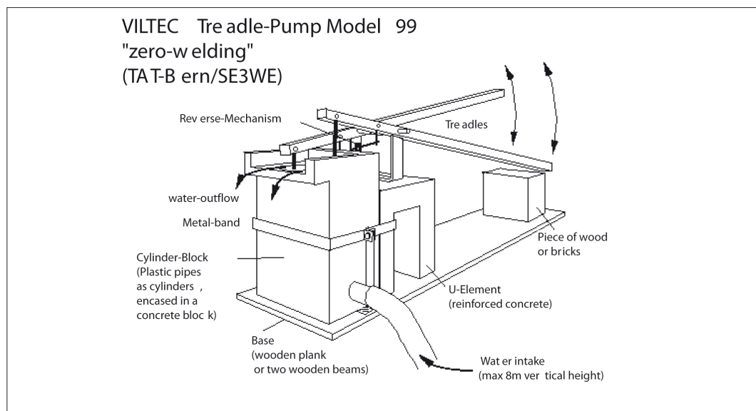
Figure 9.39: Treadle pump (Viltec treadle-pump model 99 “zero welding”).
