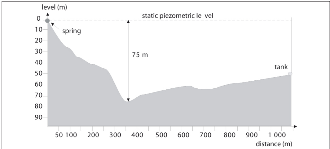
Figure 11.7: Static profile and pressure class of pipes.
