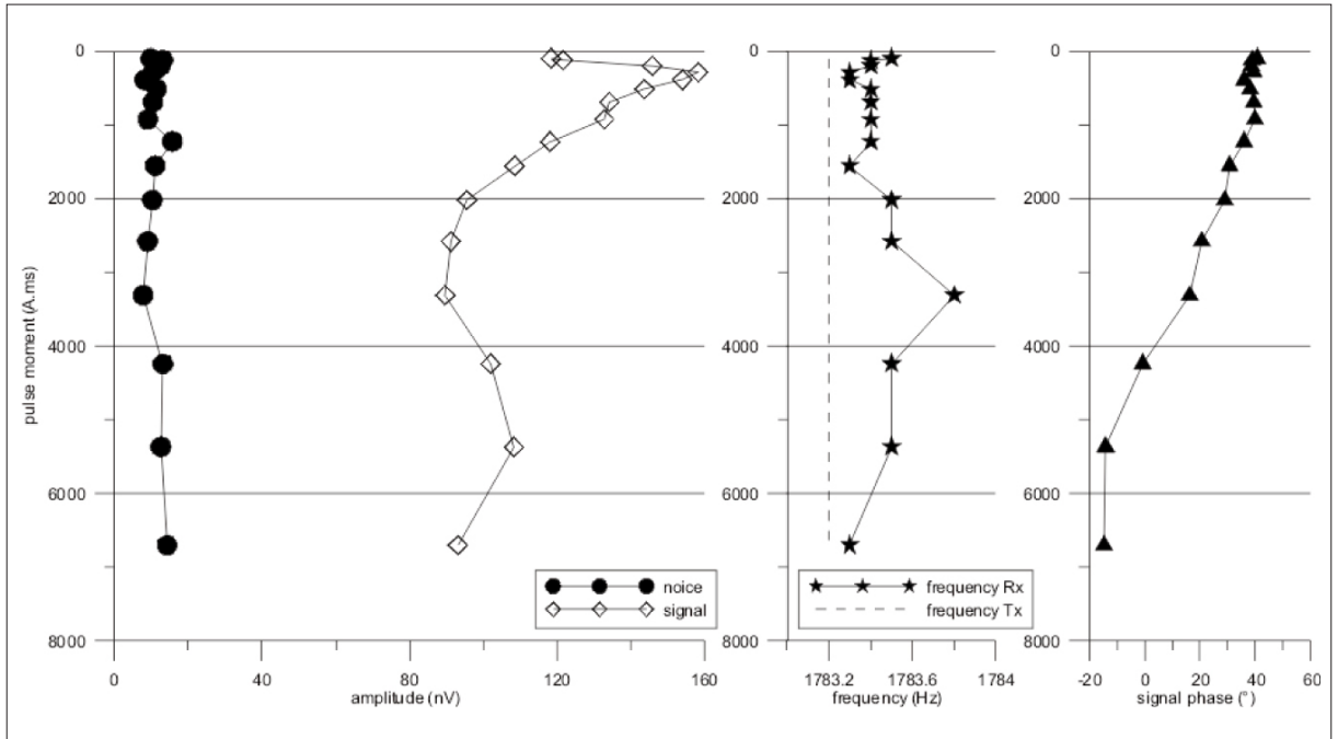
Figure 5.70: MRS raw data, ACPI school.
