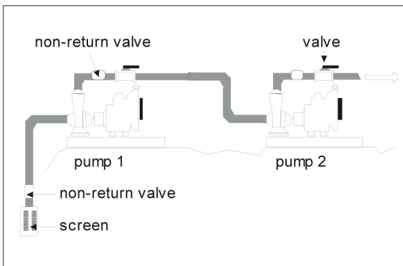
Figure 9.8: Mounting two identical pumps in series.
