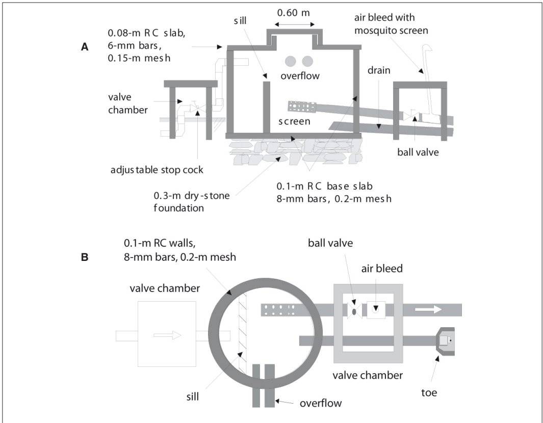
Figure 11.19: Reinforced concrete break-pressure tank.
