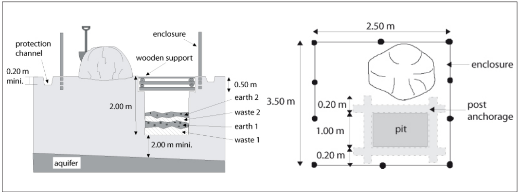
Figure 13.28: Refuse pit.
