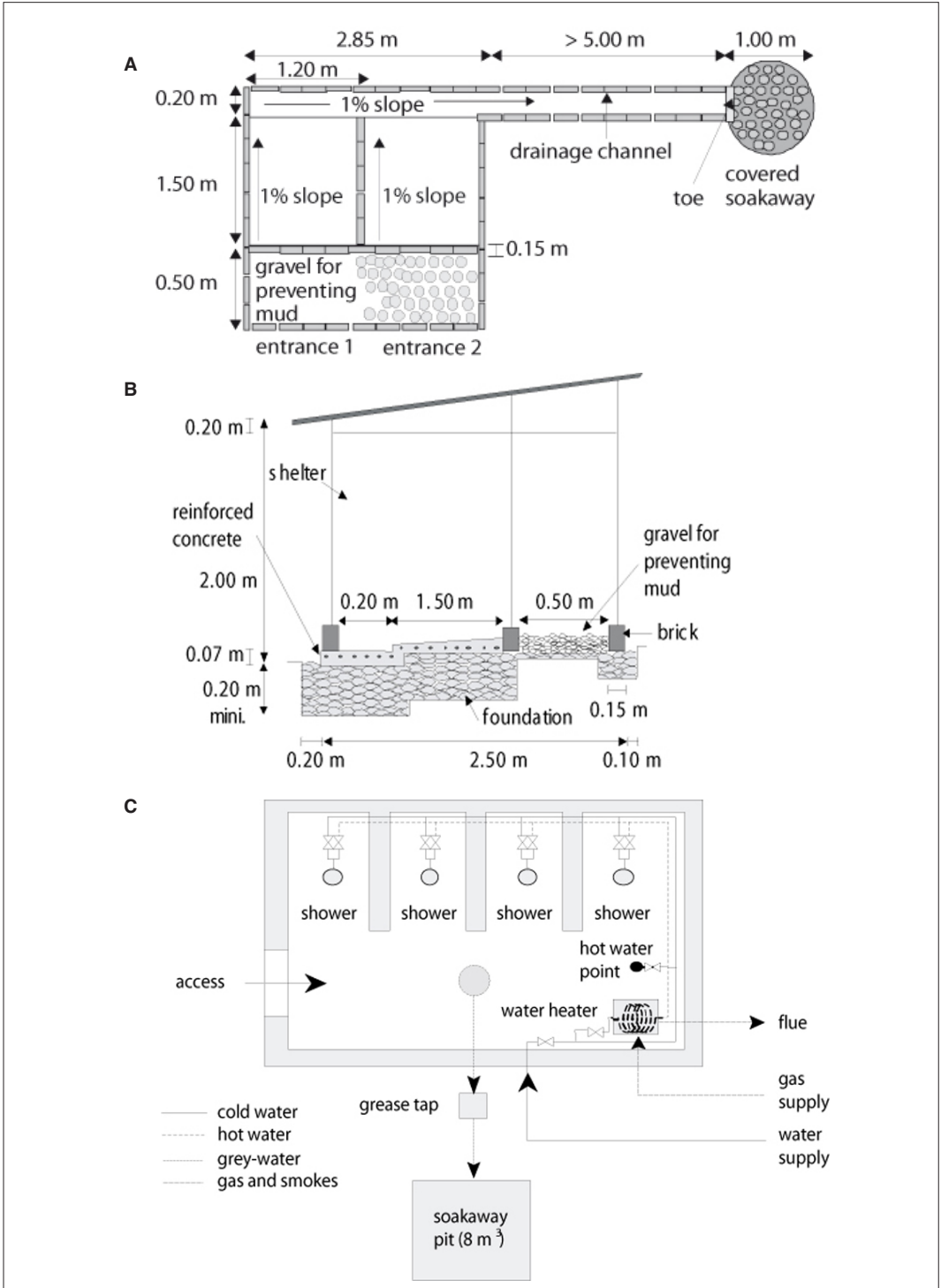
Figure 13.24: Showers.
