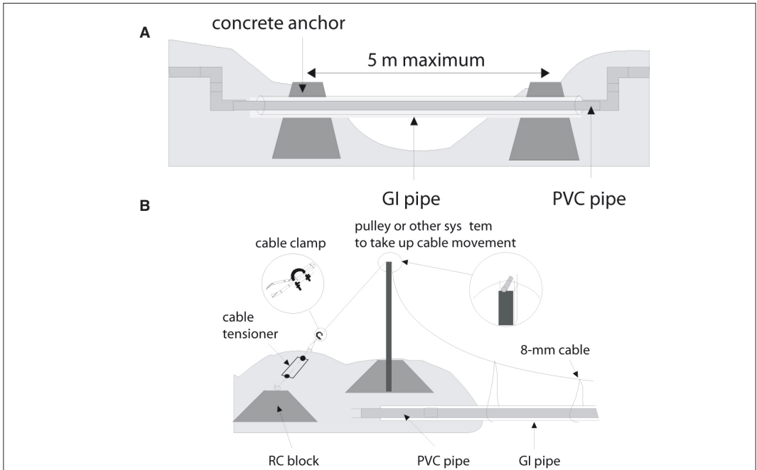
Figure 11.28: Crossing over ravines or rivers. A: use of a GI sleeve. B: suspended pipe.
