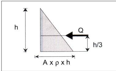
Figure 39: Ground thrust on a retaining wall.
