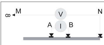
Figure 5.9: Half-Schlumberger array.
