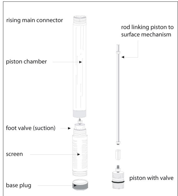
Figure 9.27: Kardia pump cylinder.
