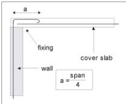
Figure 12: Reinforcement for a semi-fixed slab.
