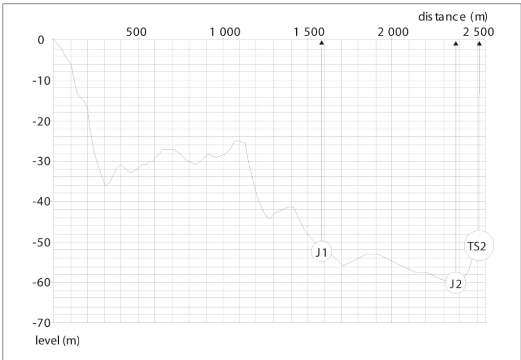
Figure 11.5A: Topographic profile (from catchment/J1/J2/Ts2, Aloua).
