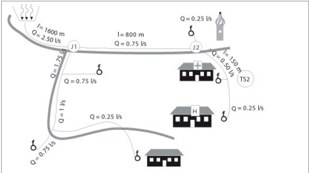
Figure 11.5B: Layout plan (from catchment/J1/J2/Ts2, Aloua).
