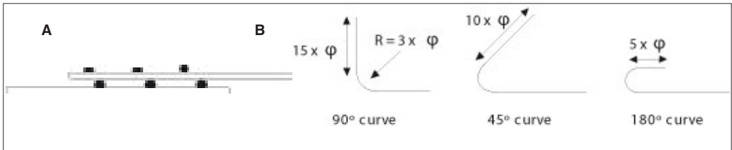
Figure 4: Arrangement of reinforcement bars.
