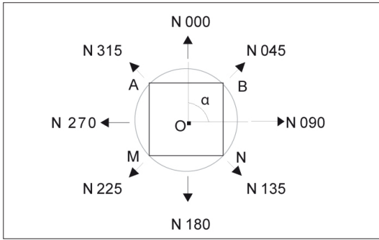
Figure 5.24: Layout for square survey.
