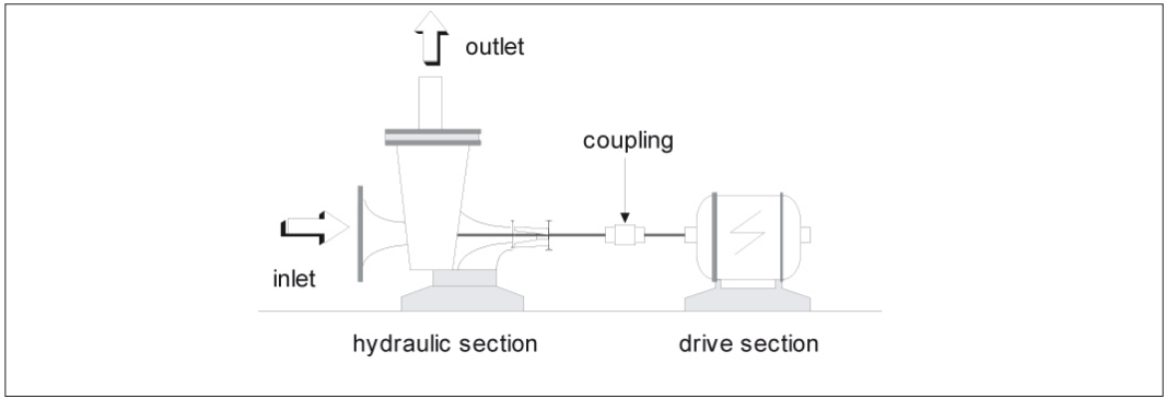
Figure 9.1: Electric centrifugal pump (surface).
