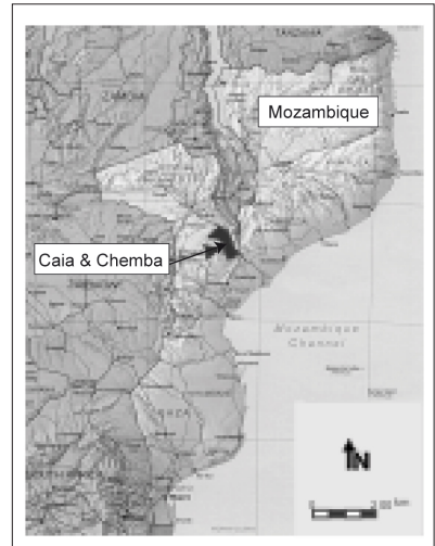
Figure 5.55: Location of the study zone in Mozambique.
