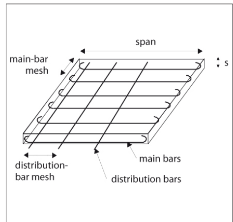
Figure 9: Reinforcement for a slab.
