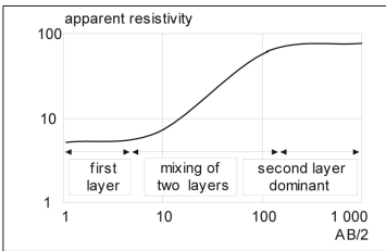
< Figure 5.21: Two-layer curve.
