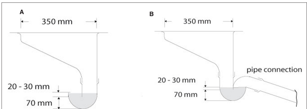
Figure 13.10: Water seal. A: placed over the pit. B: with an off-set pit.
