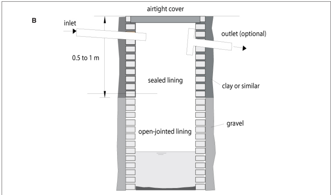
Figure 13.16: Soakaway pits. B: lined pit.
