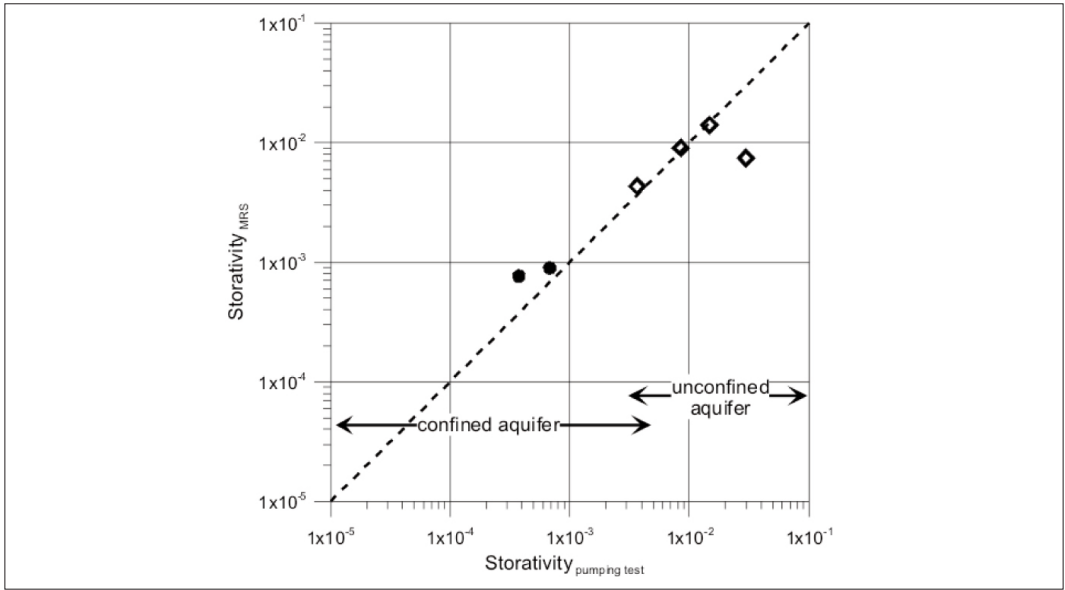
Figure 5.79: Aquifer storativity.
