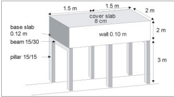
Figure 37: Elevated rectangular tank.
