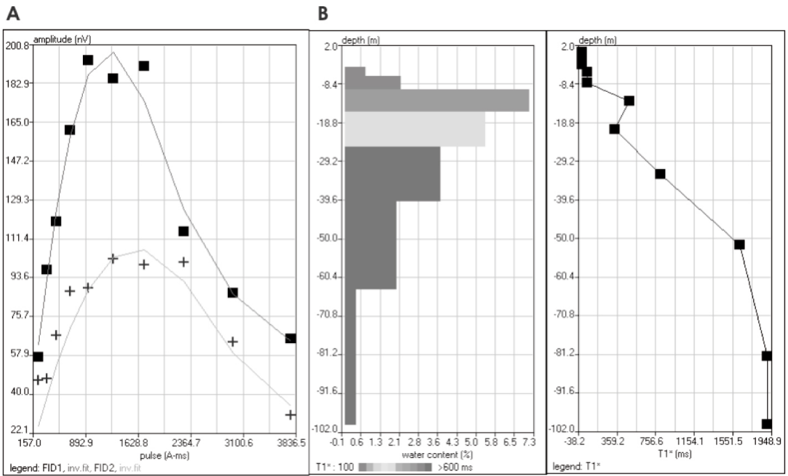
Figure 5.51: MRS curves.
