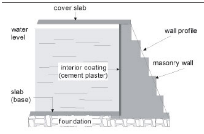
Figure 23: Tank side wall.
