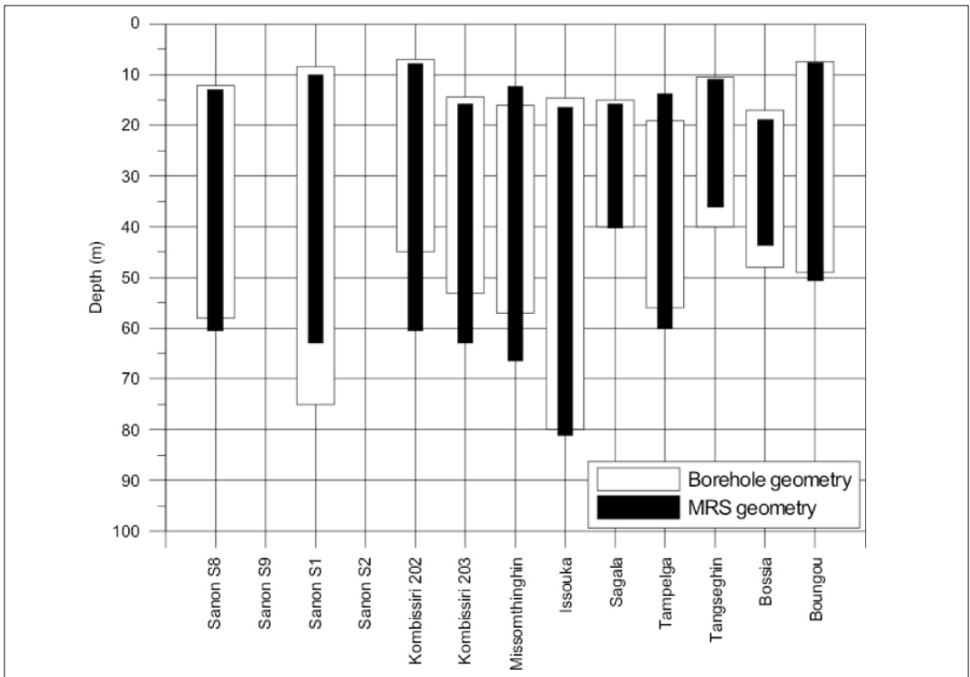
Figure 5.78: MRS and reservoir geometry.
