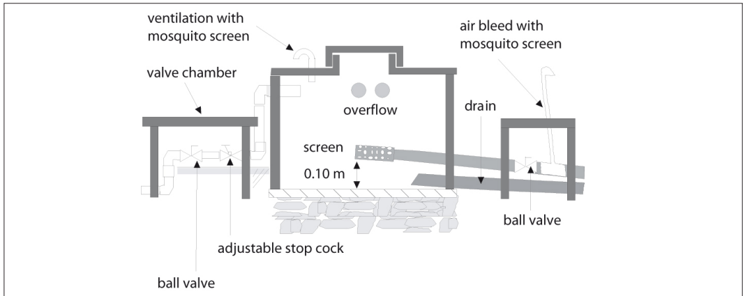
Figure 11.20: Storage tank.
