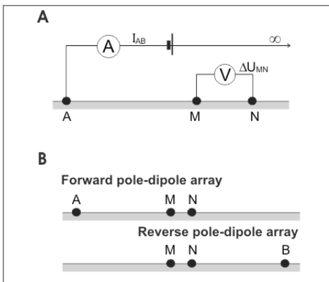
Figure 5.18: Half-Schlumberger sounding. A: principle. B: arrays.
