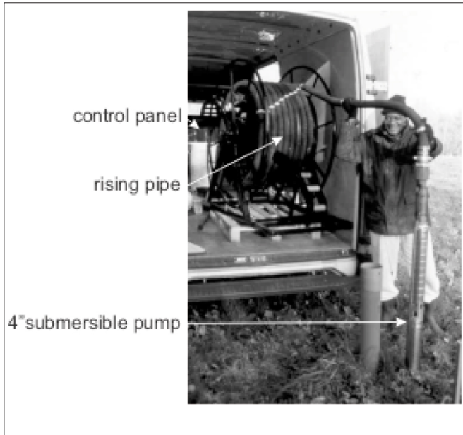
Figure 6.23: ACF pumping-test kit.
