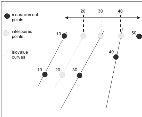
Figure 2: Isovalue method: linear variations proportional to distance.
