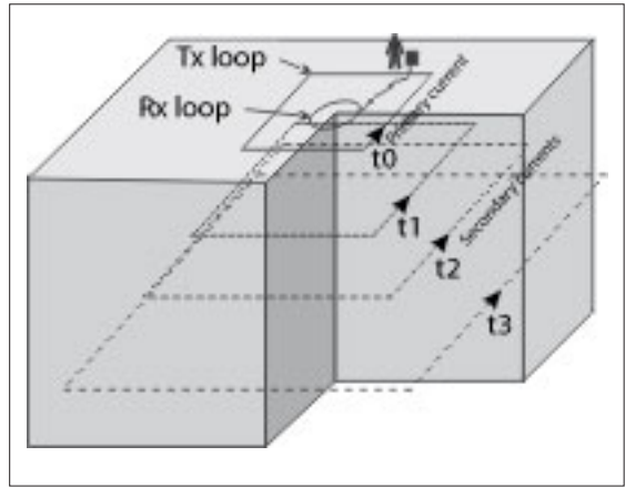
Figure 5.43: TDEM sounding principle.
