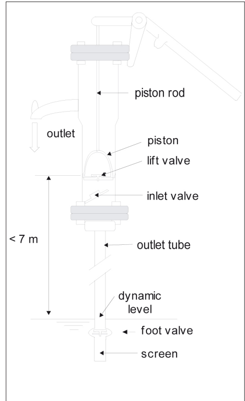
Figure 9.32: VN6-type suction pump.
