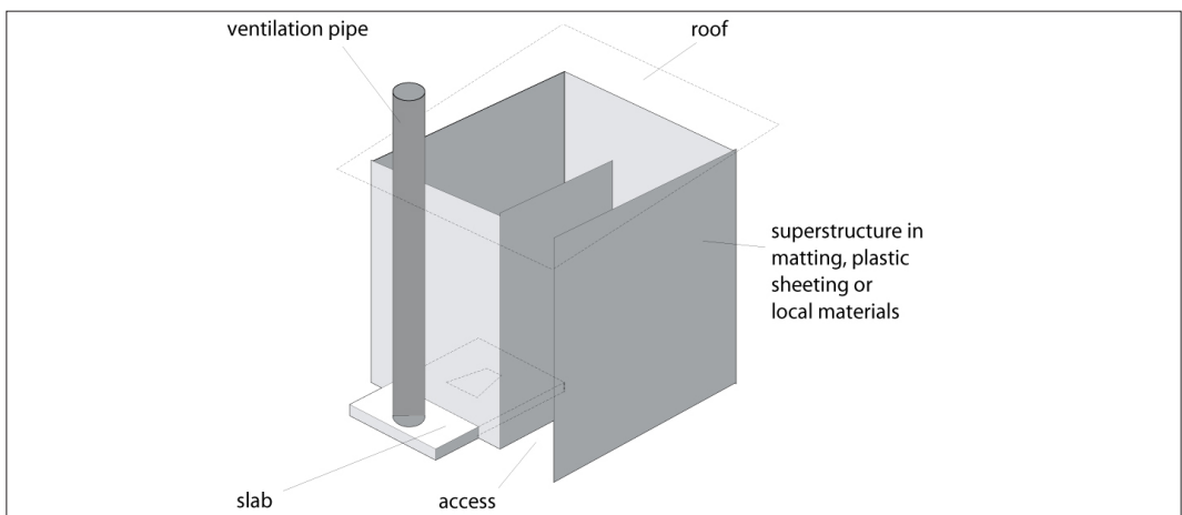
Figure 13.9: Spiral-shaped superstructure.
