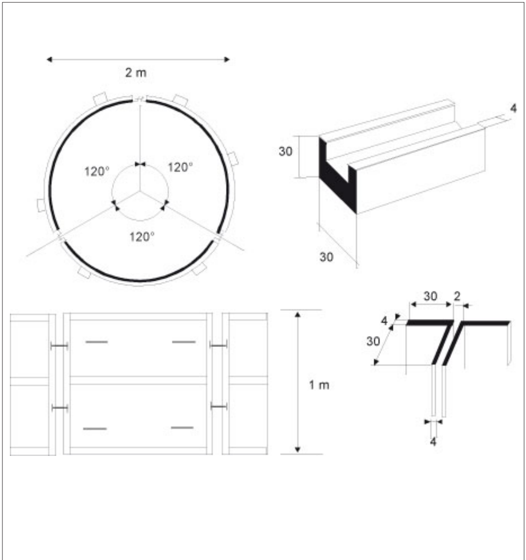
Figure 48: Shuttering for a headwall (2 m external diameter)
