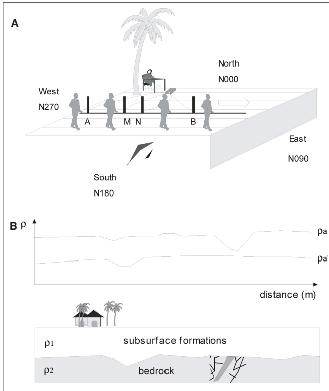
Figure 5.28: Resistivity profiling. A: setting up. B: example.
