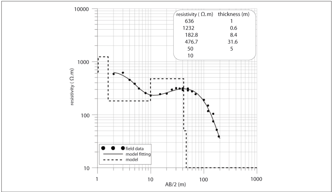
Figure 5.67: VES Schlumberger (rms = 7.5%), ACPI School.
