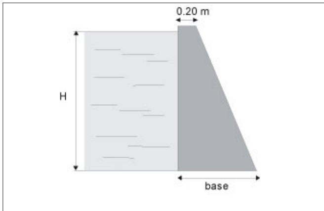
Figure 22: Retaining wall.
