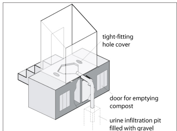
Figure 13.17: LASF design.
