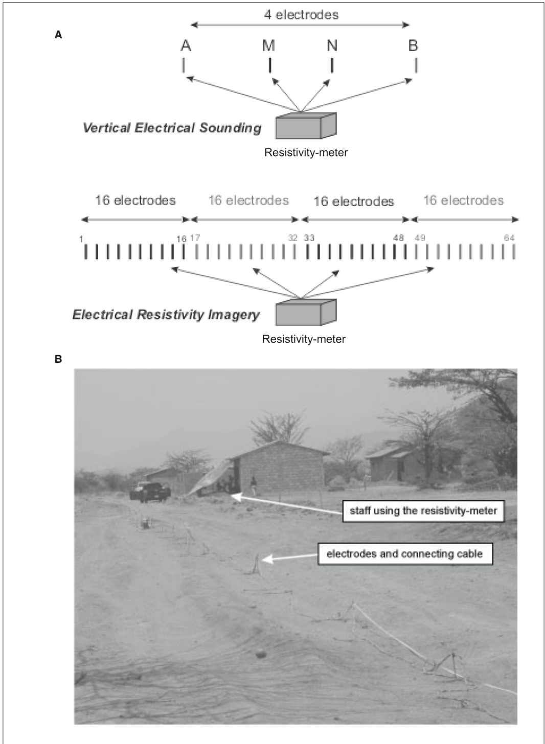
Figure 5.30: ERI measurement array.
