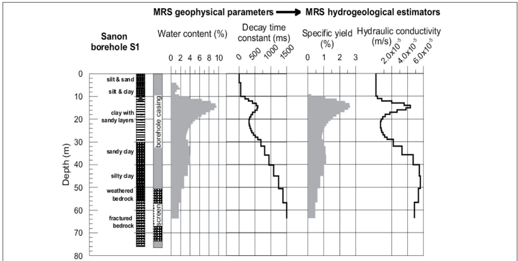
Figure 5.47: MRS geophysical parameters (the presented decay time is T_1 , see Box 5.4) and hydrogeological indicators, example of Sanon S1 Borehole in Burkina Faso, weathered granite (ACF, 2002).
