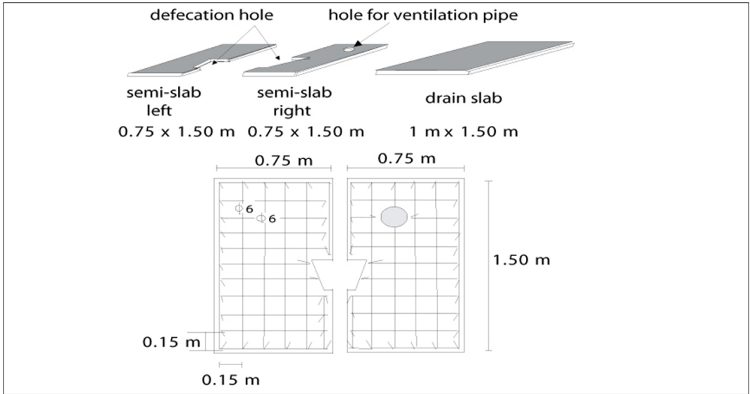
Figure 13.6: Reinforcement for a two-part symmetrical slab.
