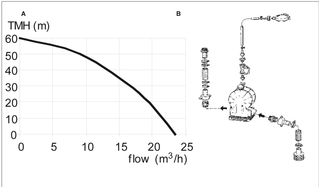
Figure 9.19: Membrane dewatering pump.
