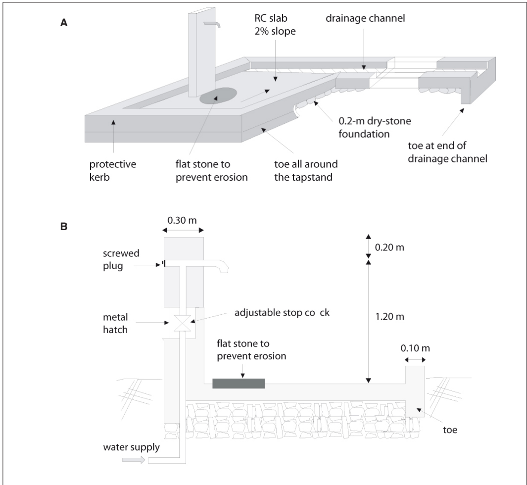
Figure 11.33: Reinforced-concrete tapstand with one tap. A: general view. B: section.
