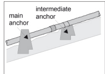
Figure 11.30: Pipe anchors.
