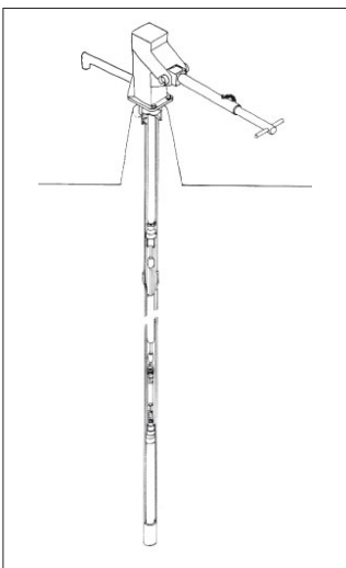
Figure 9.30: Aquadev and Afridev pumps.
