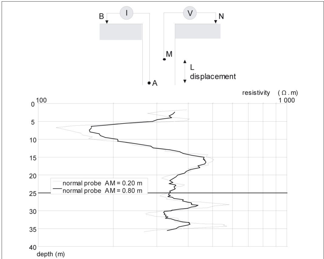
Figure 5.32: Electric logging (ACF, Siem Reap, Cambodia, 1998).
