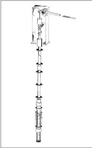
Figure 9.28: Kardia K65 and K50 pumps (for very large depths).
