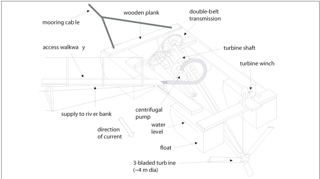
Figure 9.22: Garman pump installed on a raft.
