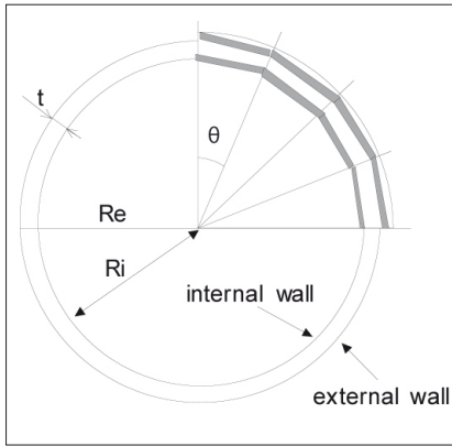
Figure 1: Shuttering for a 16-element circular tank.
