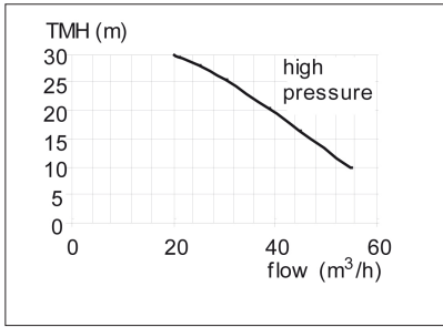
Figure 9.16: Characteristic curve for an electric dewatering pump.
