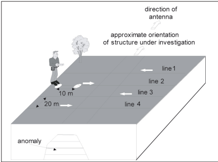
Figure 5.37: Anomaly/antenna/profile directions, VLF.
