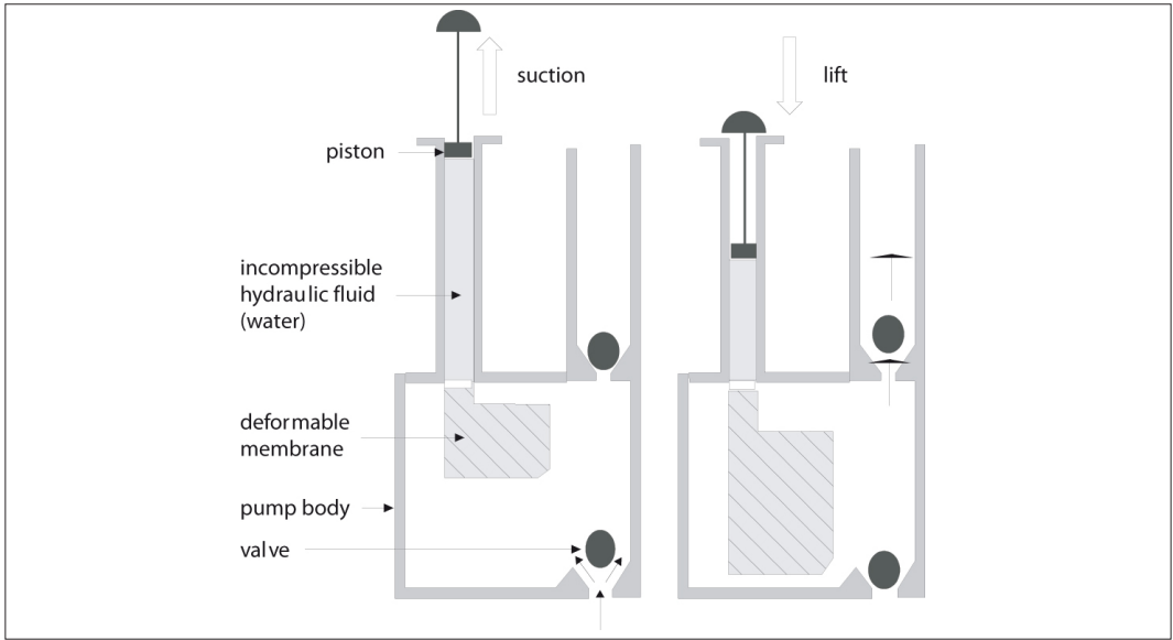
Figure 9.33: Working principle of Vergnet hydropump.
