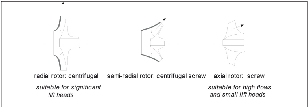
Figure 9.2: Rotor designs in turbopumps.
