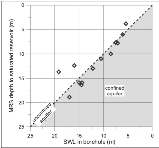
Figure 5.77: MRS and static water level (SWL).
