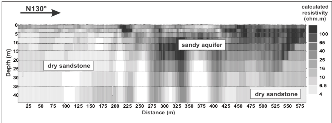
Figure 5.31: Electrical Resistivity Imagery (ACF, Mozambique, 2000).
