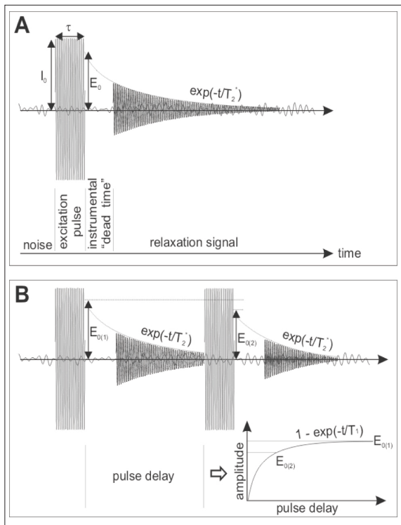
Figure 5.54: Time sequence of the MRS signal.
