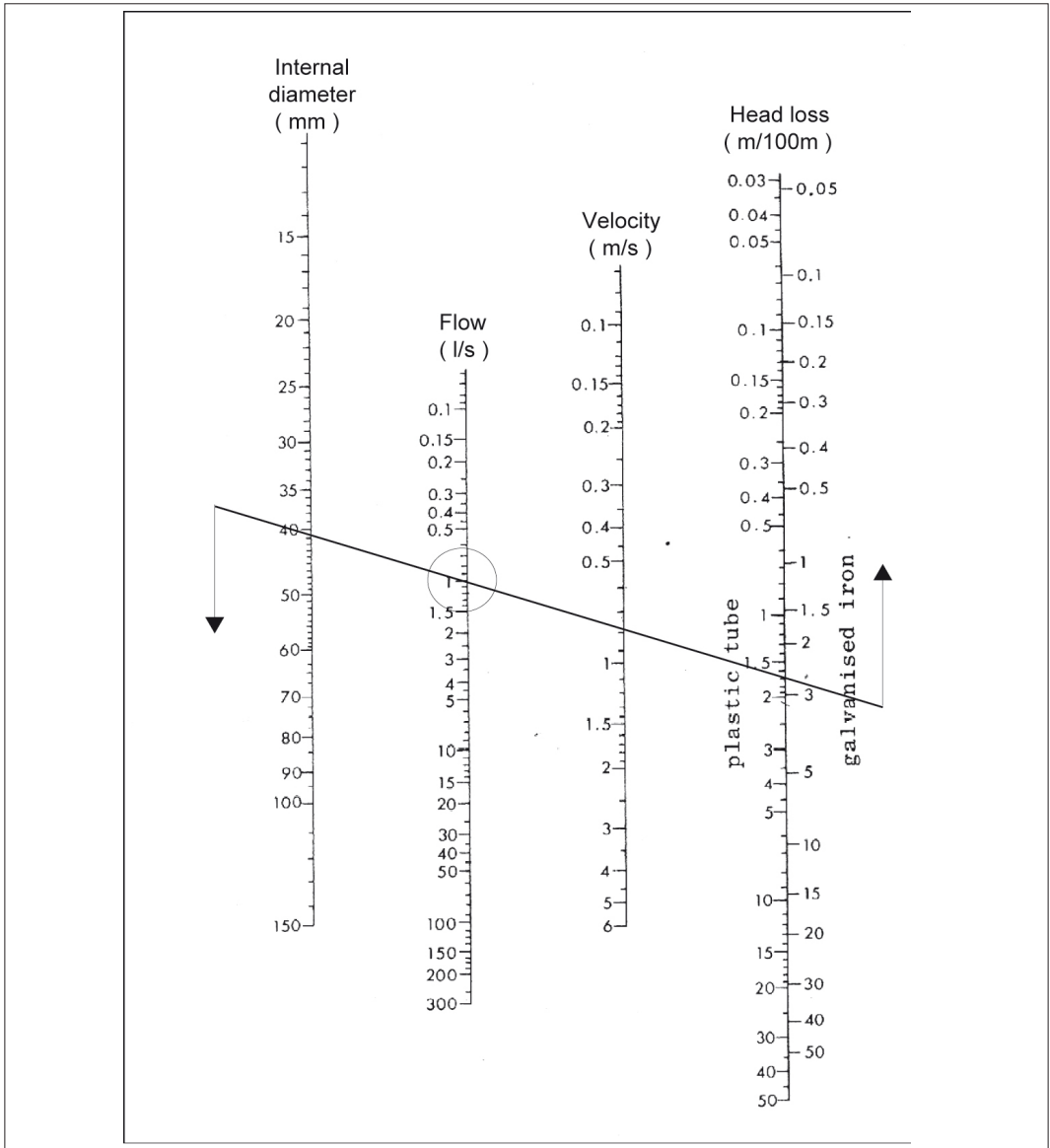
Figure 11.10: Design chart for calculating linear head-losses.
