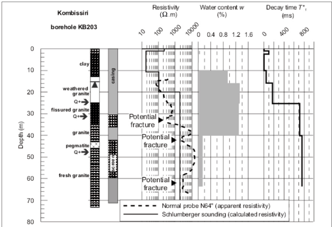
Figure 5.82: Suppression, example of Kombissiri borehole #203.
