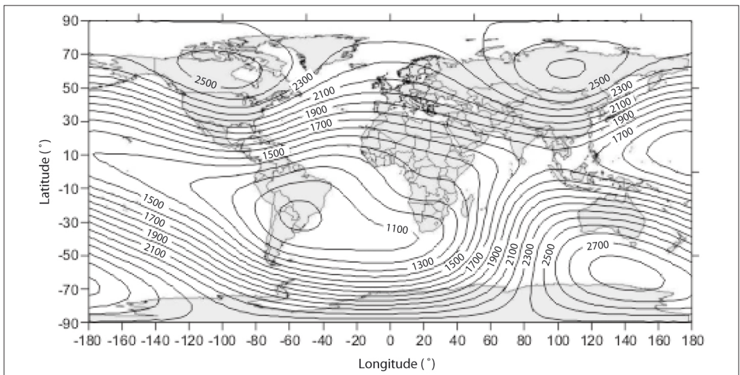
Figure 5.50: Theoretical Larmor frequency, year 2002 at sea level.
