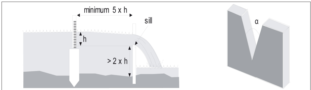
Figure 3.4: Thin-plate weir.
