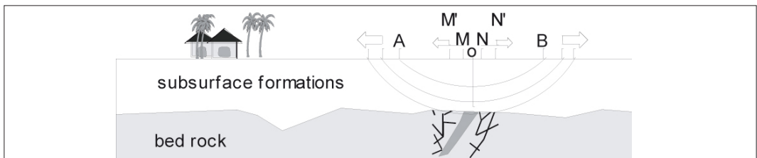
Figure 5.15: Implementation of Schlumberger VES.
