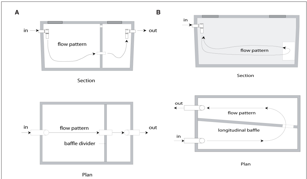
Figure 13.13: Septic tank flow pattern (adapted from Crites & Tchobanoglous, 1998). A: interior baffle placed across tank. B: interior baffle placed longitudinally.
